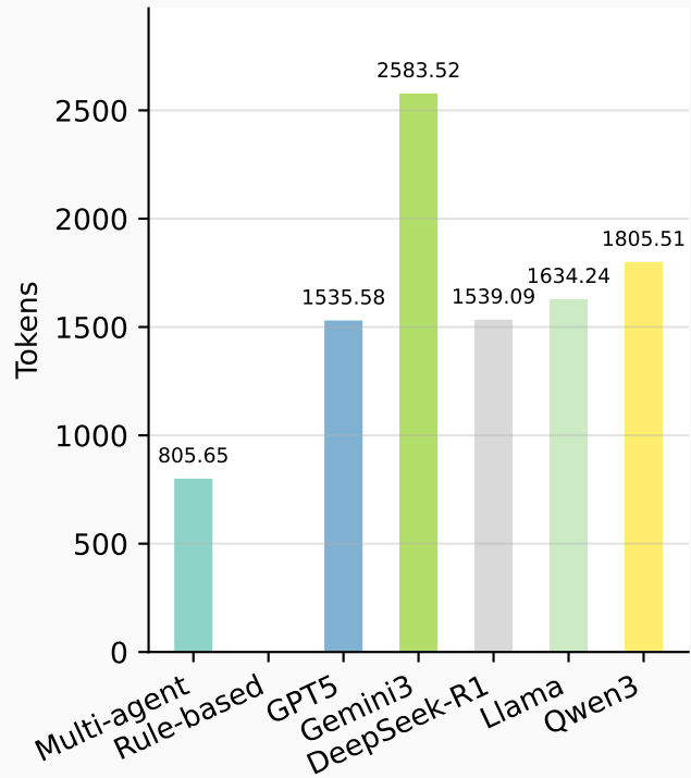
(c) Tokens
