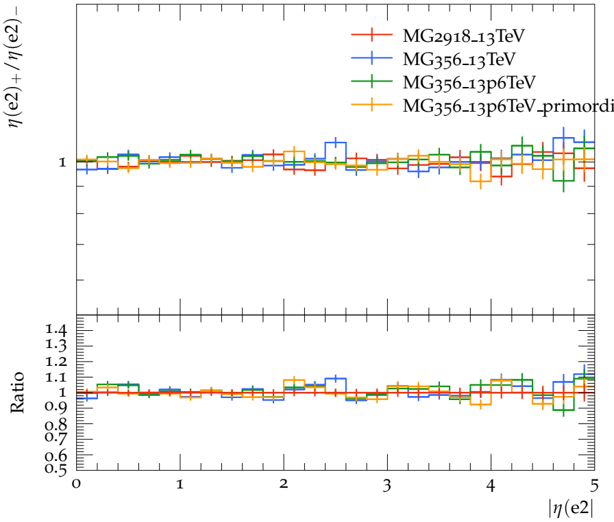
Pseudorapidity +/- ratio of second electron
