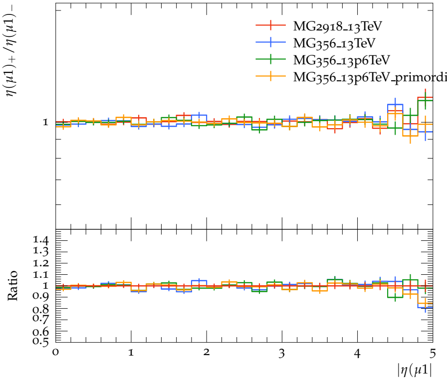
Pseudorapidity +/- ratio of first muon
