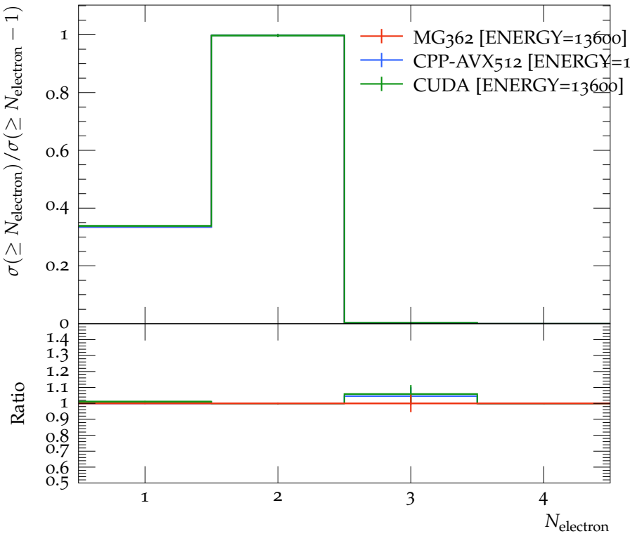
Ratio of prompt electron multiplicity
