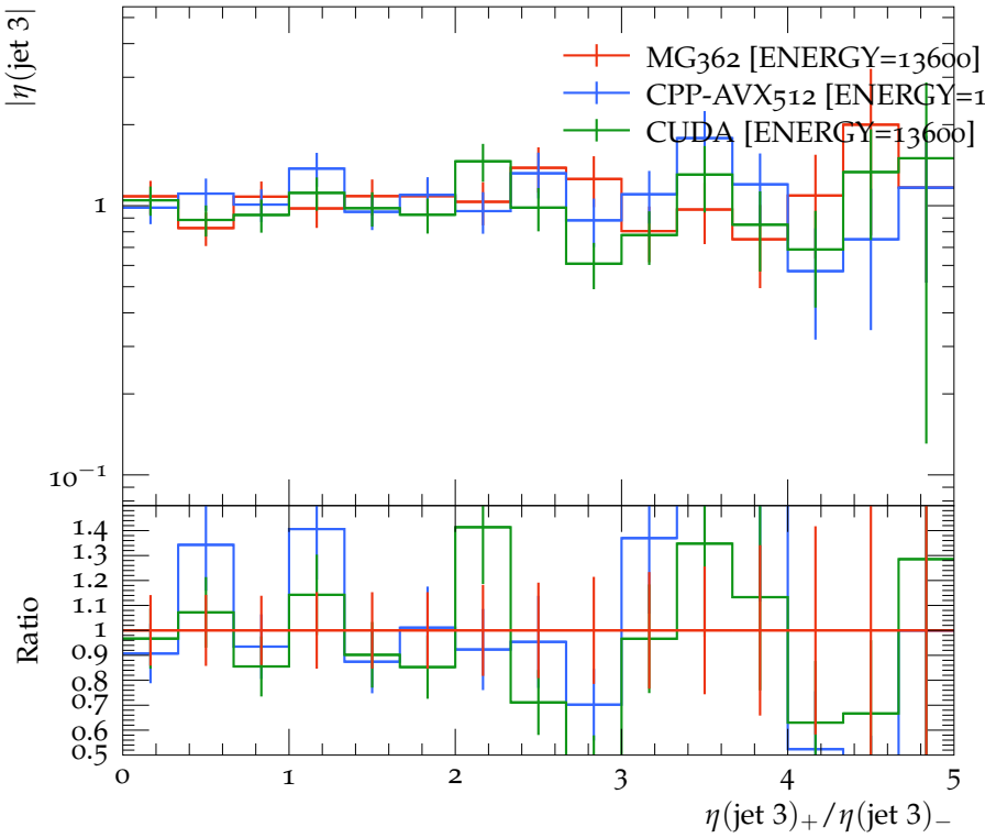
Pseudorapidity + / - ratio of third jet
