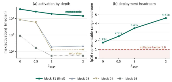
Fig. 2 Dose-response of alignment-loss weight on last-block activation magnitude (seed and LR schedule fixed, 5,000 steps, 799 images, evaluation resolution)
