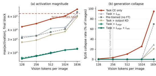
Fig. 1 Last-block activation magnitude (a) and fp16 generation collapse rate (b) versus vision tokens per image, for five controlled variants and the pre-trained model. The dashed line in (a) is the fp16 limit (65,504); the vertical line marks the training and evaluation resolution. 1,836 is the token budget for the native 1,600x900 nuScenes frame (1,824 tokens realized).
