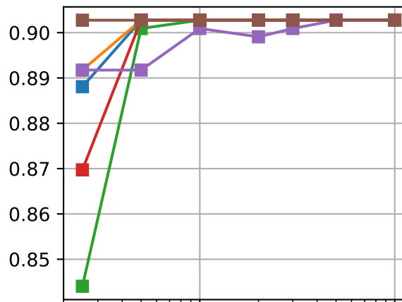
ACC tails
