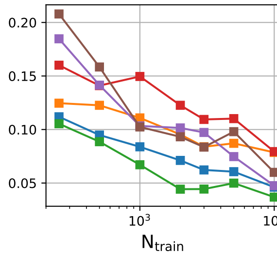
WD tails
