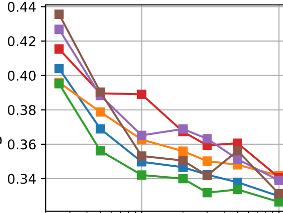
LogLoss tails
