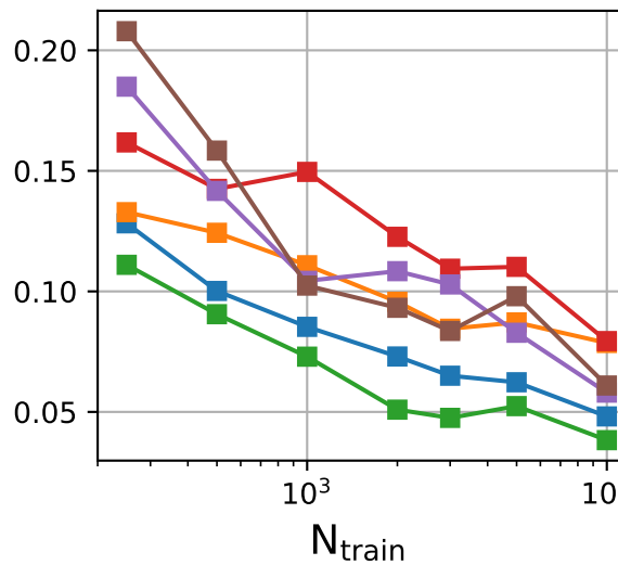
Z tails
