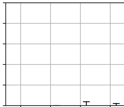
Maximum depth = 2
