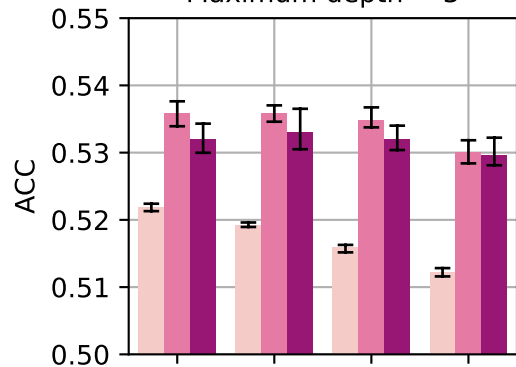
Maximum depth = 3
