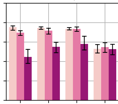
Maximum depth = 6
