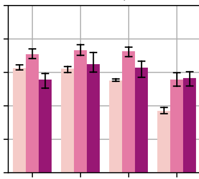
Maximum depth = 4
