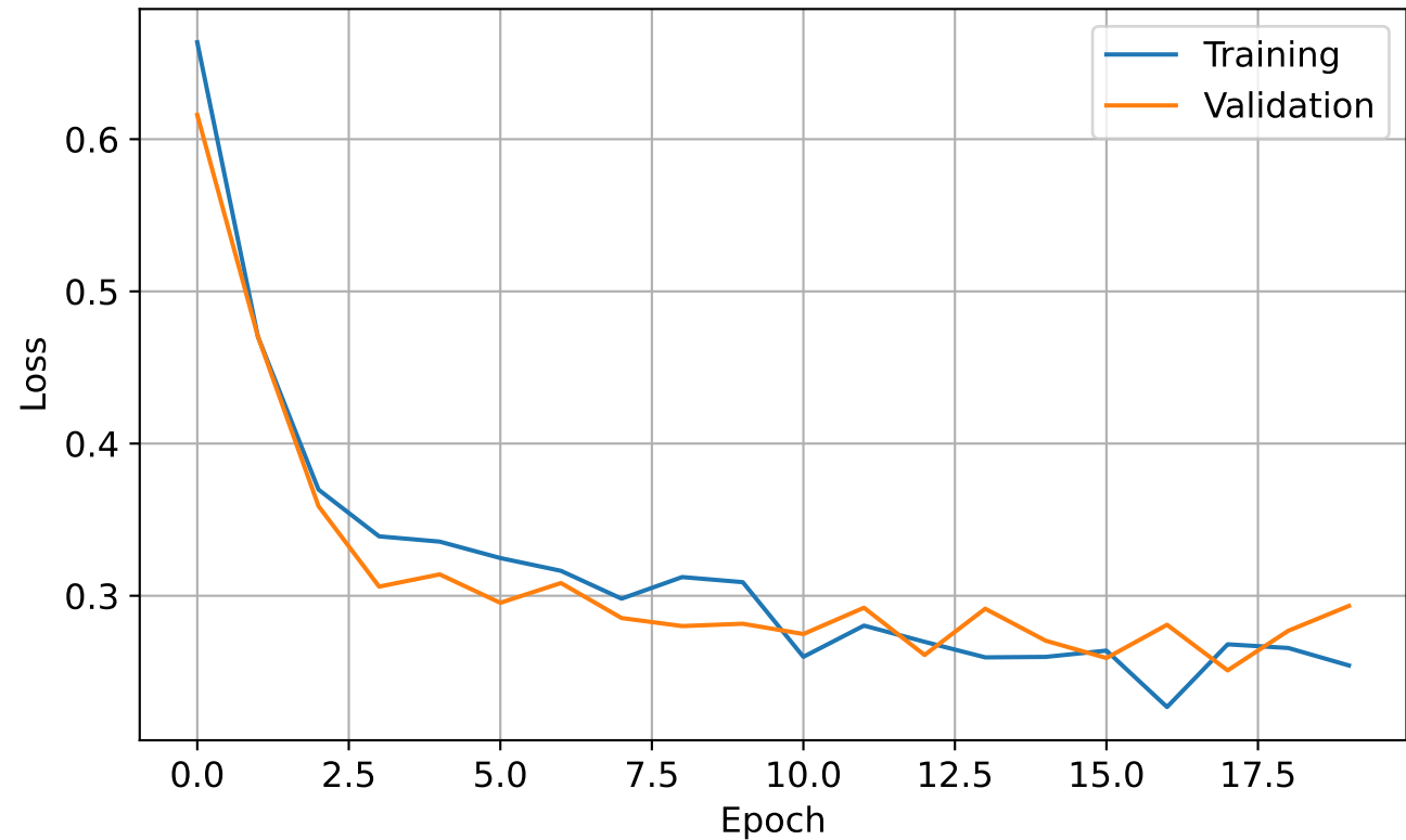
Model Loss
