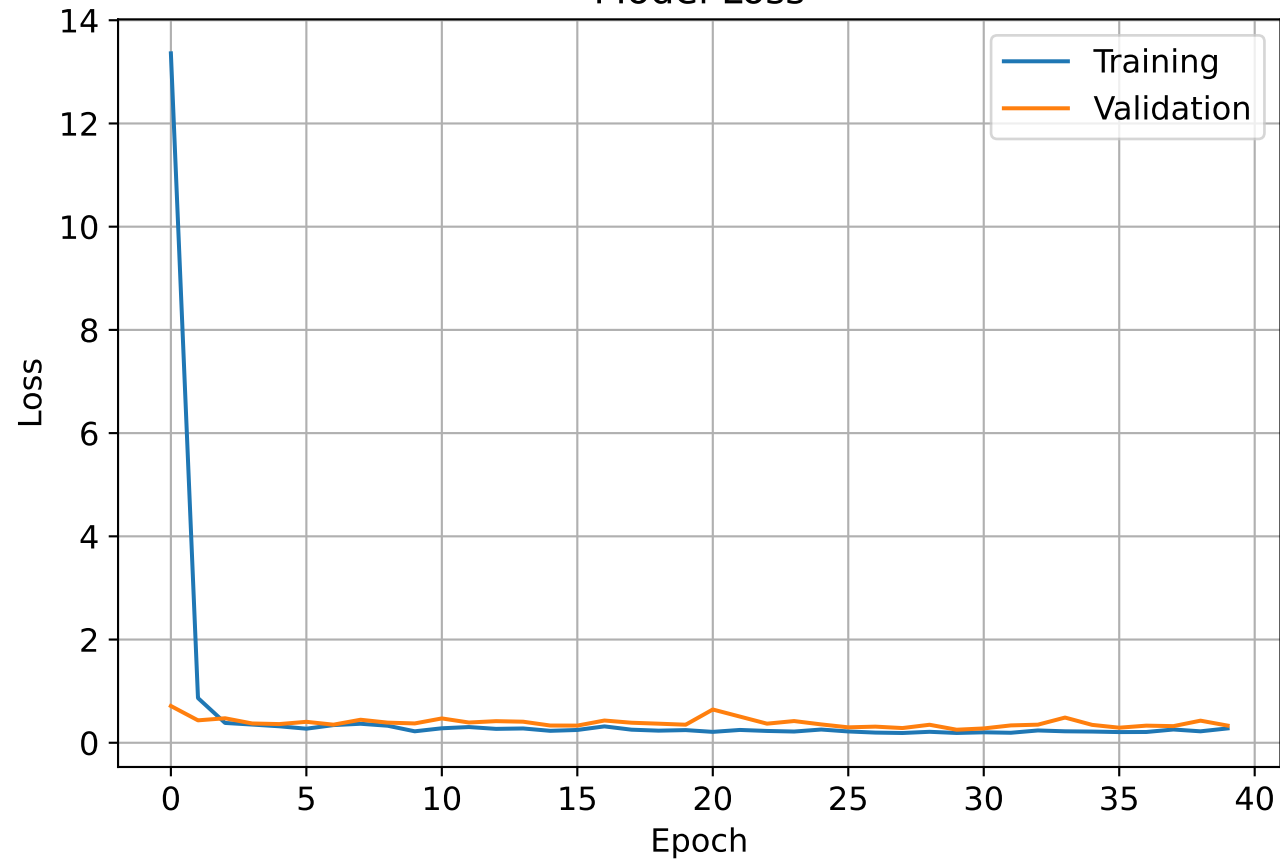
Model Loss
