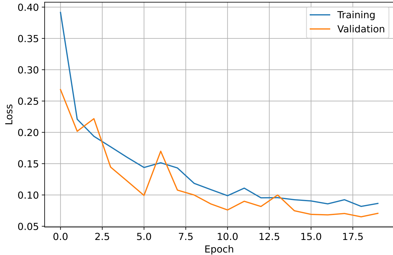
Model Loss
