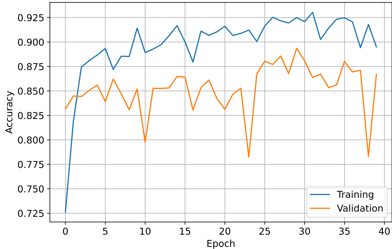
Model Accuracy
