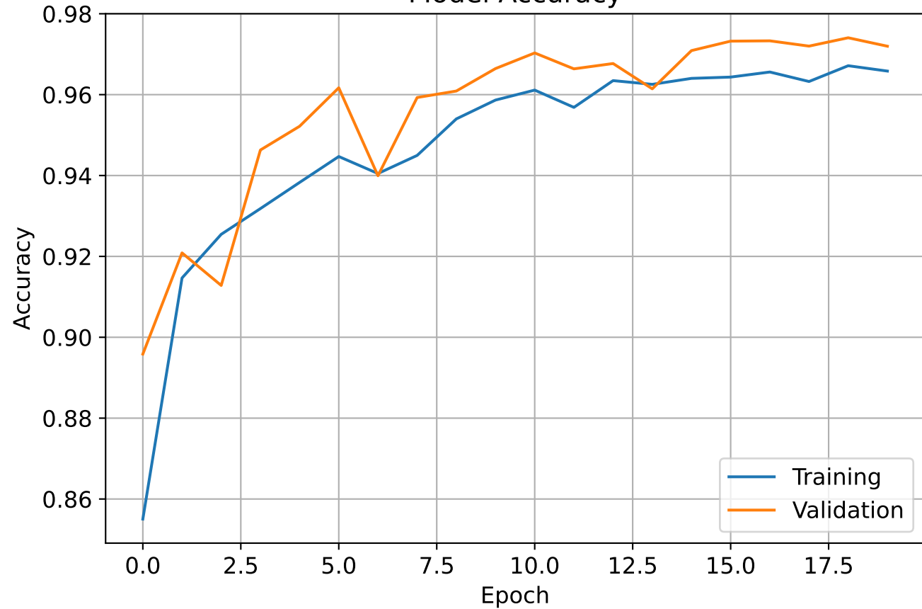
Model Accuracy
