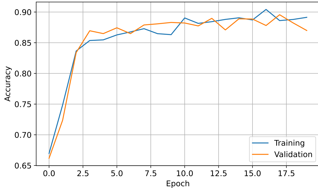
Model Accuracy
