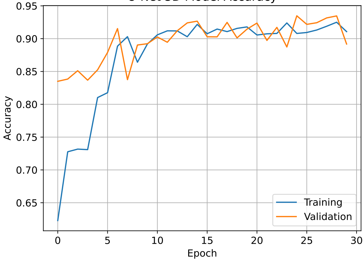
U-Net 3D Model Accuracy
