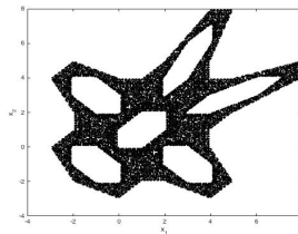
Figure 2: 20000 iterates
