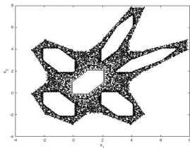
Figure 1: 10000 iterates
