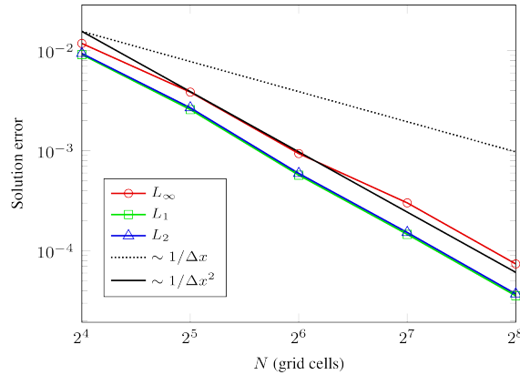
Fig. 6.3.2: Spatial convergence rates for two-dimensional coaxial cable geometry.
