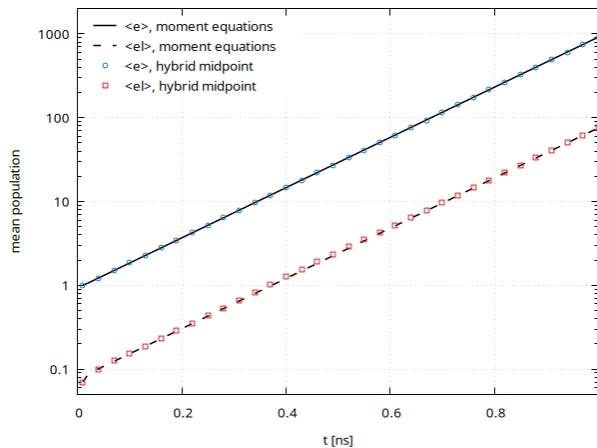
Fig. 4.4.3: Mean populations for the stiff two-group model, hybrid midpoint tau leaping against the moment equations.
