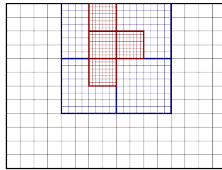
Fig. 3.1.7: Classical cartoon of tiled patch-based refinement. Bold lines indicate entire grid blocks.
