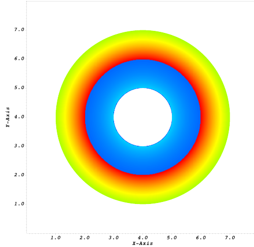
Fig. 6.3.1: Field distribution for a coaxial cable geometry on a 512^2 grid.
