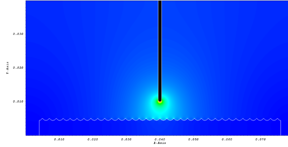
Fig. 6.3.3: Field distribution for a profiled surface geometry on a 2048^2 grid.
