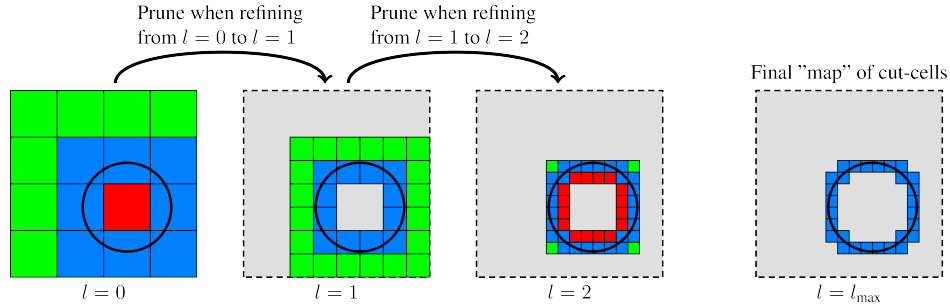
Fig. 3.1.5: Pruning cut-cells with the signed distance field. Red-colored grid patches are grid patches entirely contained inside the EB. Green-colored grid patches are entirely outside the EB, while blue-colored grid patches contain cut-cells.
