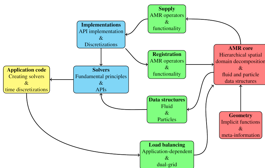
Fig. 2.1.1: Concept design sketch for chombo-discharge .
