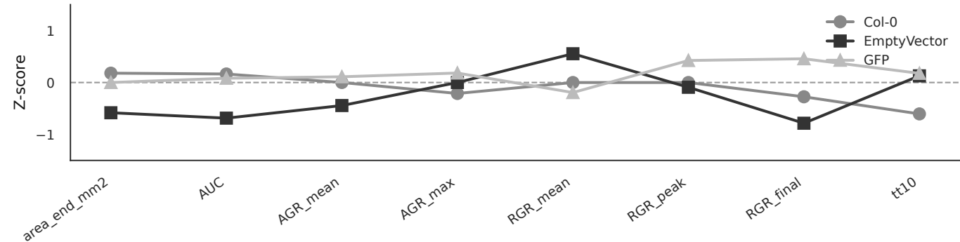
Root: Control z-profiles (pooled baseline)
