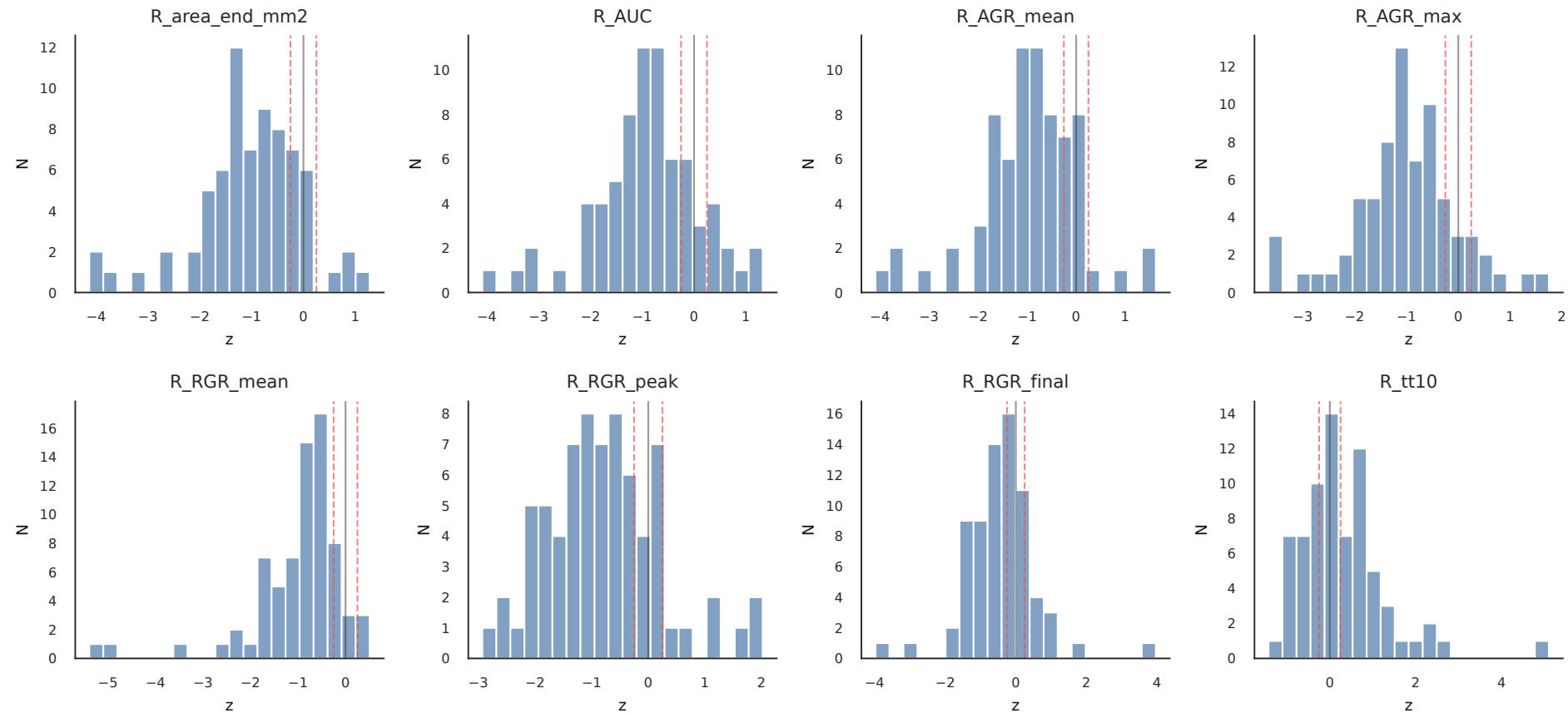
Root: Effector z-distributions (white band = noise |z| < 0.25 )
