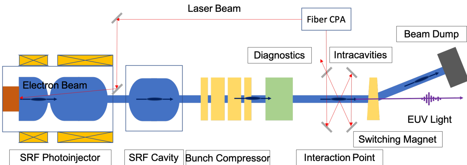
Figure 1: Inverse Compton Scattering EUV Light Source Layout
