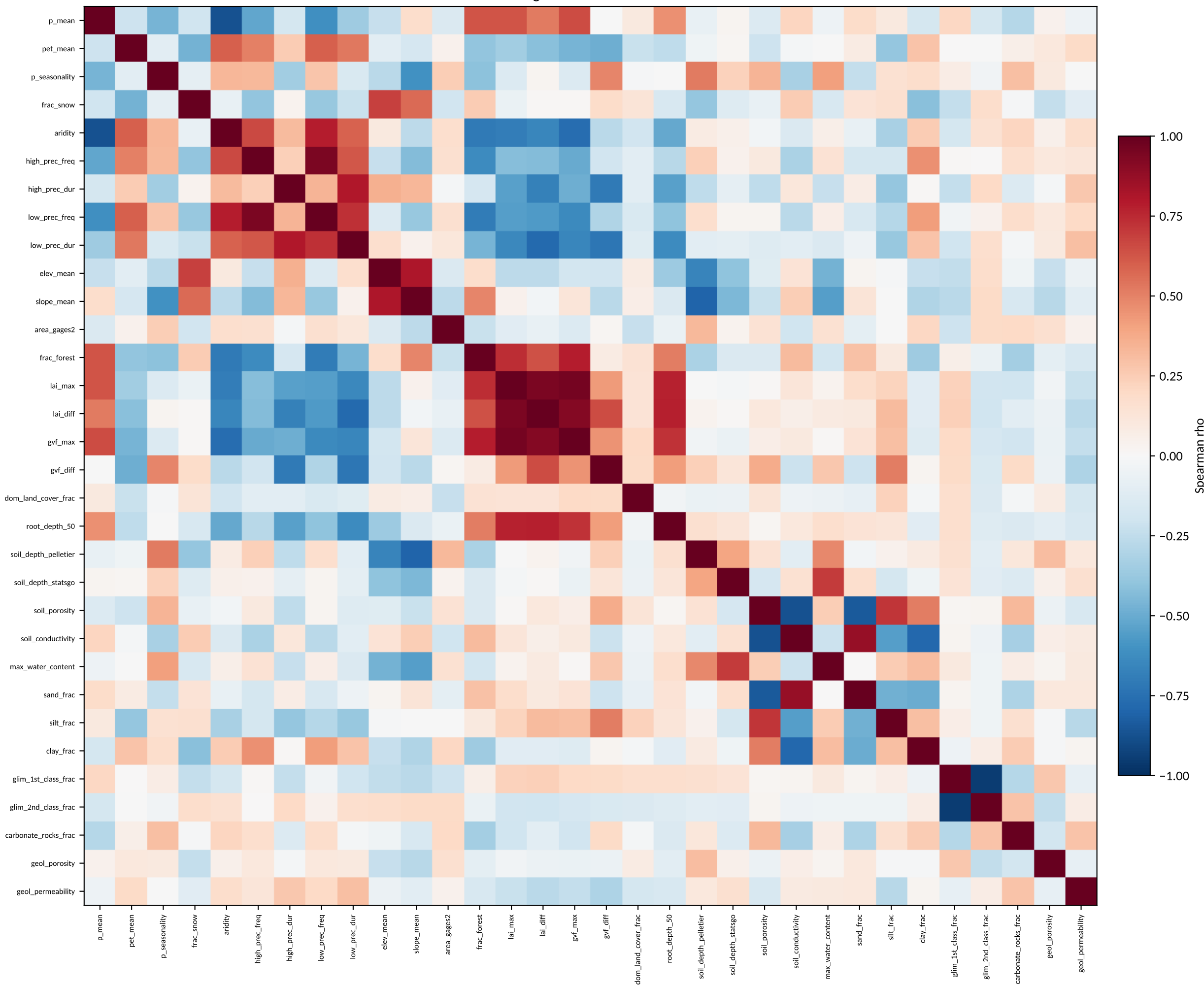
Spearman correlation of 32 continuous CAMELS attributes Categorical codes excluded
