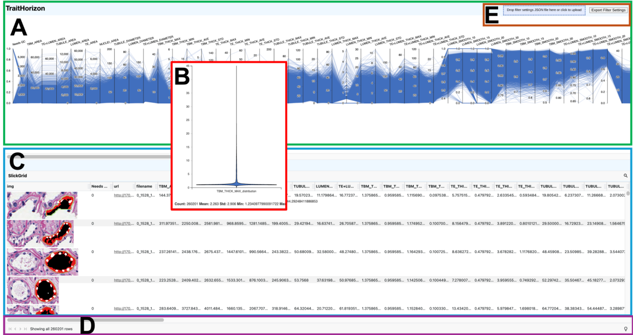
Figure 1: TraitHorizon web application interface. (A) The interactive parallel coordinates plot displays 99 pathomic features from 260,201 tubules, wherein each blue line represents one tubule feature vector. (B) A violin plot shows the value distribution of a selected feature when hovered over. (C) The data grid presents each segmented tubular image, with the original PAS-stained tubule on the left and the segmentation overlay on the right (green: tubular basement membrane; white: tubular nuclei; black: tubular lumen; red: tubular epithelium). Associated feature data loaded from the TSV (e.g., filename and corresponding feature values) are also displayed. (D) The bottom status bar shows the number of instances currently visible. (E) The drop zone and export button allow users to save filter configurations and filtered row IDs. TraitHorizon allows users to customize which columns are included or excluded in the parallel coordinates plot. Here, the URL and filename columns were excluded from the parallel coordinates plot but are shown in the data grid.
