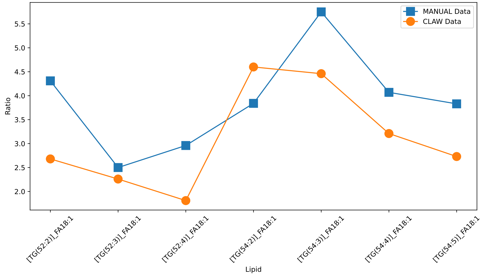
CLAW vs Manual Degummed Area Ratio
