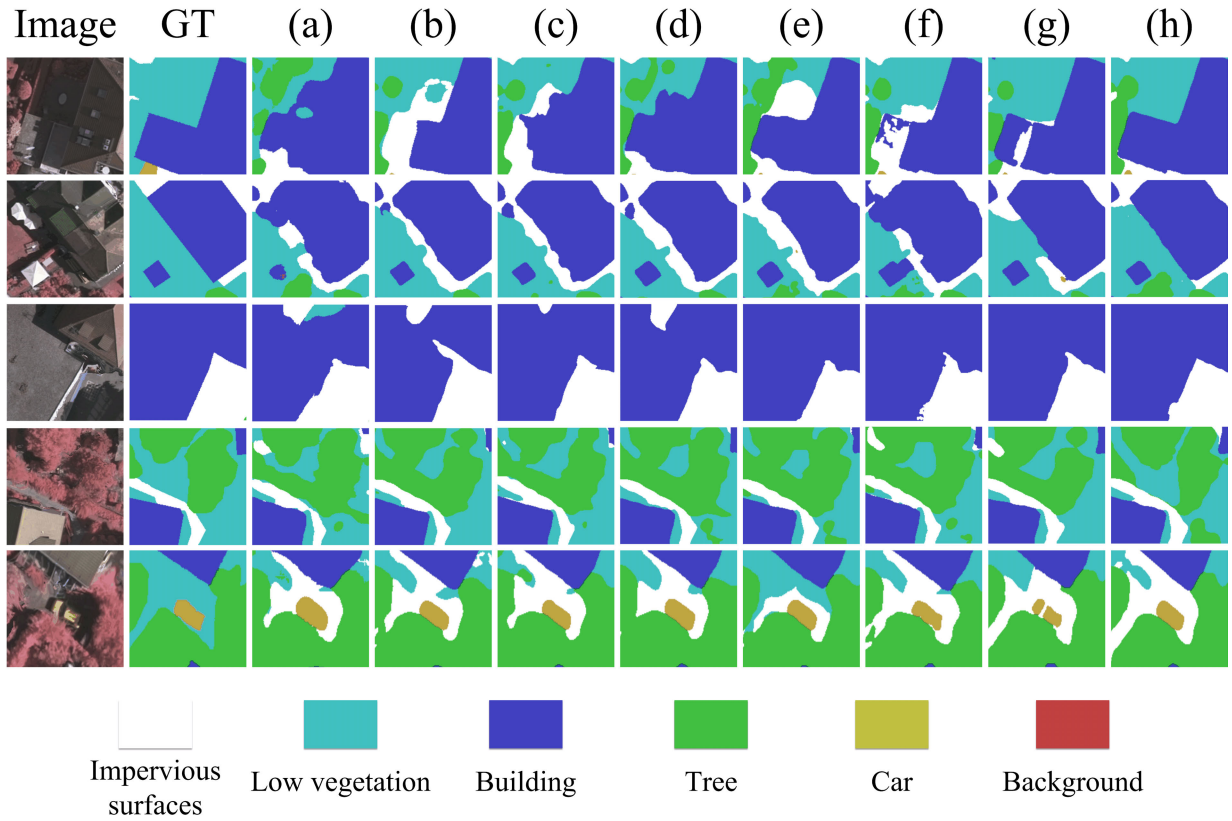
Fig. 15. Local enlargement of segmentation results on the Vaihingen dataset for SFFNet and other comparative models. (a) Corresponds to ABCNet. (b) Corresponds to MResU-Net. (c) Corresponds to A2-FPN. (d) Corresponds to ST-Unet. (e) Corresponds to dc-Swin. (f) Corresponds to MPCNet. (g) Corresponds to Xnet. (h) Corresponds to SFFNet (Ours). From the figure, it can be observed that our model performs better in segmenting areas with large grayscale variations compared to spatial segmentation methods while also having more comprehensive spatial information compared to purely frequency domain segmentation methods.
