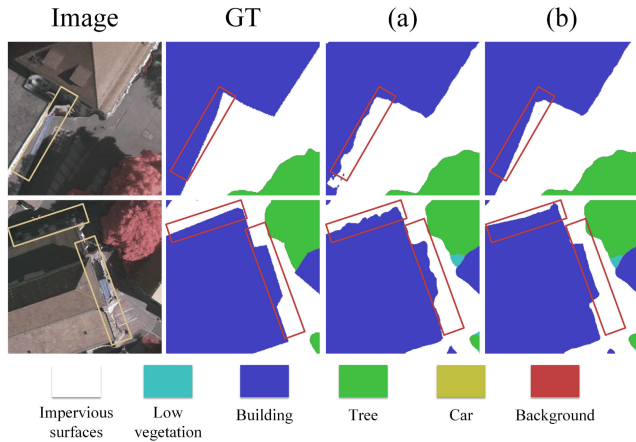
Fig. 11. Local enlarged segmentation results before and after adding low-frequency features to the baseline. (a) Corresponds to the baseline. (b) Corresponds to Baseline + WTFD-L. It can be seen that using low-frequency features has a noticeable effect on objects that are difficult to segment under shadows.
