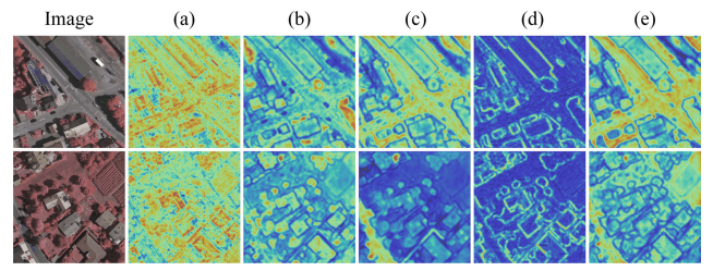
Fig. 13. Effects of four types of feature mappings on the extracted features in the first stage. (a) Shows the original features before mapping. (b) Shows the features after local mapping. (c) Shows the features after global mapping. (d) Displays the decomposed high-frequency features. (e) Shows the decomposed low-frequency features. It can be observed that local features focus more on local details, such as small objects, while global features focus on large-scale continuous regions. High-frequency features primarily focus on local edges, and low-frequency features also emphasize large-scale continuous regions, but they tend to pay more attention to shadowed areas and regions with multiple textures compared to spatial global features. However, spatial features lack attention to shadowed areas and regions with multiple textures.
