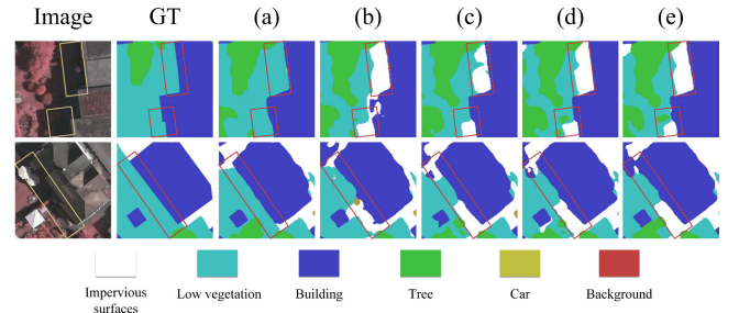
Fig. 8. This figure shows the locally enlarged segmentation results of removing various components in SFFNet. (a) Represents SFFNet. (b) Represents SFFNet without the global branch. (c) Represents SFFNet without the local branch. (d) Represents SFFNet without WTFD-L. (e) Represents SFFNet without WTFD-H. It can be observed from the figure that removing any branch results in a decline in segmentation performance.
