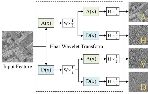
Fig. 5. Diagram illustrating the principle of feature decomposition using the Haar wavelet transform. Here, A(x) represents low-pass filtering of the original data to obtain low-frequency approximation coefficients, while D(x) represents high-pass filtering of the original data to obtain high-frequency detail coefficients. Each decomposition halves the length or the width of the features. The proposed WTFD in this article obtains the low-frequency signal A , horizontal high-frequency signal H , vertical high-frequency signal V , and diagonal high-frequency signal D through two iterations of the Haar wavelet transform.
