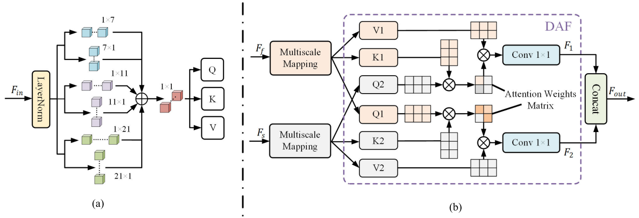
Fig. 6. MDAF structure. (a) Multiscale mapping. (b) MDAF. This structure is used for semantic alignment and feature selection between frequency domain features and spatial domain features. We first perform multiscale mapping on both types of features to align them to a unified scale. Then, utilizing a DAF implemented with cross-attention, we facilitate interaction and selection between the two types of features. Finally, the selected features are combined to obtain more representative feature signals for subsequent segmentation.
