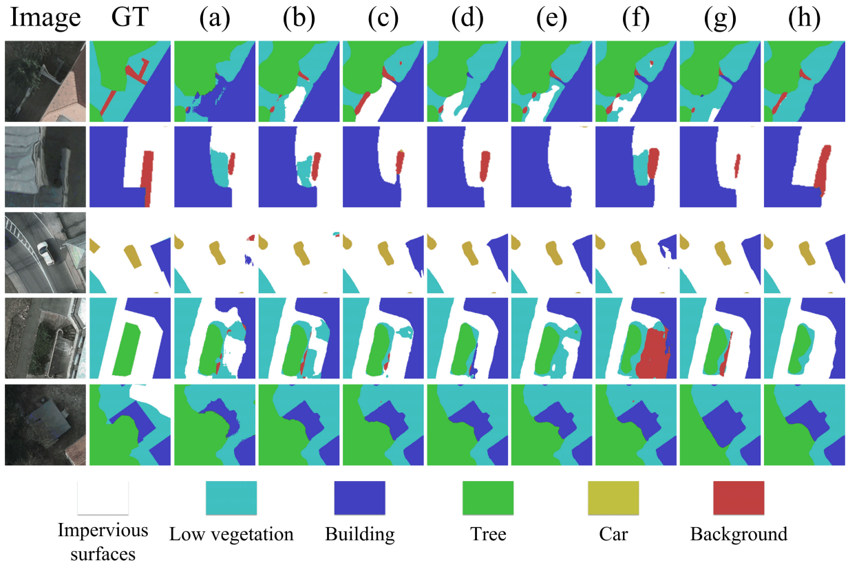
Fig. 18. Local enlarged view of segmentation results of SFFNet and other comparative models on the Potsdam dataset. (a) Corresponds to ABCNet. (b) Corresponds to MAREsU-Net. (c) Corresponds to A2-FPN. (d) Corresponds to ST-Unet. (e) Corresponds to dc-Swin. (f) Corresponds to MPCNet. (g) Corresponds to Xnet. (h) Corresponds to SFFNet (ours). Similar to the results on the Vaihingen dataset, it can be observed from the figure that our model performs better in segmenting areas with large grayscale variations compared to spatial domain segmentation methods, while compared to purely frequency domain segmentation methods, SFFNet also preserves more comprehensive spatial information.
