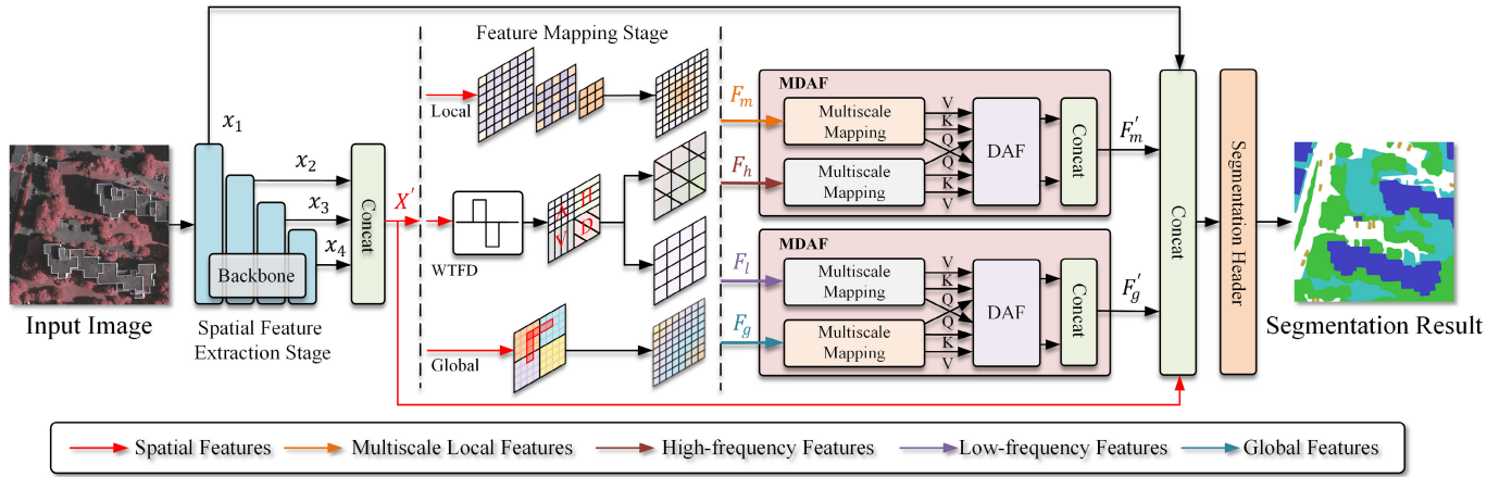
Fig. 2. This figure illustrates the main architecture of SFFNet. SFFNet is a two-stage segmentation network. In the first stage, it extracts spatial domain features to obtain sufficient spatial information. Then, in the second stage, it performs various feature mappings, including global features, local features, and frequency domain features. For frequency domain feature mapping, we introduce a module called WTfD. This module utilizes the Haar wavelet transform to decompose features into low-frequency (A), horizontal high-frequency (H), vertical high-frequency (V), and diagonal high-frequency (D) components. These components are then mapped into low-frequency features and high-frequency features. Finally, global features are combined with low-frequency features, and local features are combined with high-frequency features. To bridge the semantic gap between spatial domain features and frequency domain features, we design a feature alignment module called MDAF. This network effectively integrates spatial information into remote sensing image segmentation and enhances performance using frequency domain features, achieving excellent segmentation results even in regions with significant grayscale variations.
