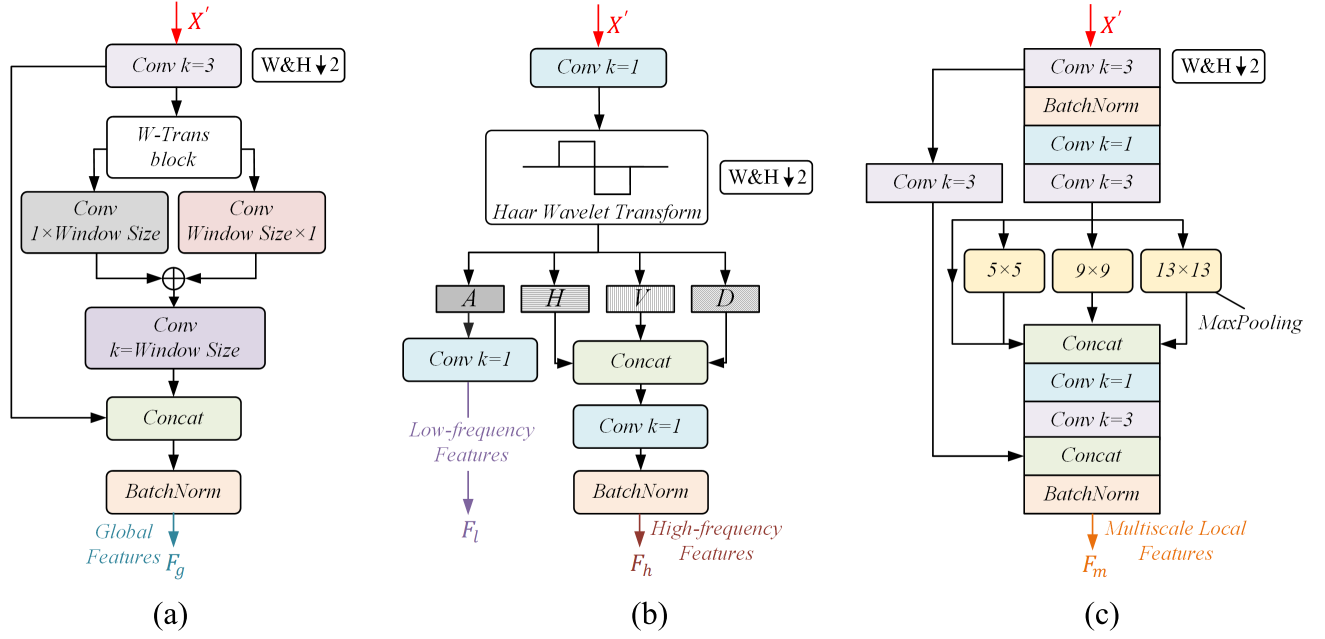
Fig. 3. This figure illustrates three feature mapping methods in the feature mapping stage. We labeled the layers where the feature size was reduced to half of its original size. (a) Represents the global branch, which is used to map the original features into global features. This module replaces the shift window in swin transformer with vertical bar-shaped convolutions, enabling the improved module to have efficient global modeling capabilities and better adaptability to remote sensing tasks. (b) Represents the WTFD, which is used to provide frequency domain information for the network. This structure first maps the original features into low-frequency component A, horizontal high-frequency component H, vertical high-frequency component V, and diagonal high-frequency component D through the Haar wavelet transform. The low-frequency component is then mapped into low-frequency features through convolution, and the three different directional high-frequency components are combined into a new high-frequency component, which is then mapped into high-frequency features. (c) Represents the local branch, which utilizes pooling pyramids to map the original features into spatially local multiscale features.
