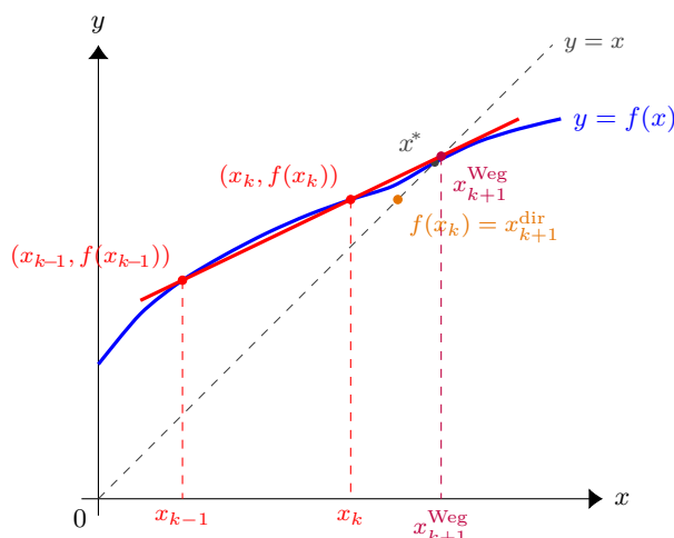
Figure 35: Geometric construction of one Wegstein step. Two prior iterates lie on the curve y=f(x) as (x_{k-1}, f(x_{k-1})) and (x_k, f(x_k)) . Their secant line (red) approximates f locally as an implicit linear model; the next iterate x_{k+1}^{\text{Weg}} is where this secant crosses the fixed-point diagonal y=x . Direct substitution would jump only as far as f(x_k) along the diagonal (orange) — visibly short of x^* — while the secant extrapolation lands almost exactly on the fixed point. For a linear f the secant coincides with the curve and Wegstein hits x^* in one step; for the non-linear f shown, the secant is a chord and one step gets within \sim 2\% of the root.
