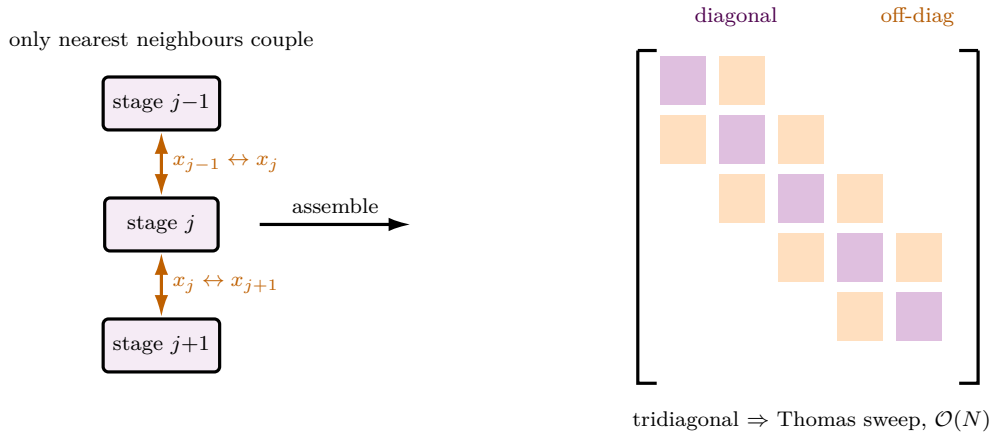
Figure 66: Why a column’s component balance is tridiagonal . Around stage j the steady balance ties only three liquid compositions — x_{j-1} descending in, x_j leaving, x_{j+1} rising in (one species shown). Because each stage couples to just its two neighbours , stacking the N balances gives a matrix with non-zeros only on the main diagonal and the two adjacent ones: a banded, tridiagonal system, one per component. Such a system is solved exactly by the Thomas algorithm in a single forward-then-backward sweep at \mathcal{O}(N) cost — no general matrix inversion — which is what Wang–Henke’s inner step and the absorber cascade both exploit. The simultaneous MESH Newton keeps the same band structure in its Jacobian, which is why even the rigorous column stays cheap per iteration.
