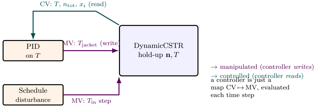
Figure 84: How a controller couples to a dynamic unit op, the Choupo Controller contract. The unit ( DynamicCSTR ) exposes a set of controlled variables the controller may read — here the reactor temperature T , total holdup, and composition x_i (green, “measurements”) — and a set of manipulated variables a controller may write each step ( T_{\text{jacket}} , T_{\text{in}} , F_{\text{in}} ; violet). A PIDController reads T and writes T_{\text{jacket}} to hold setpoint; a degenerate ScheduleController ignores the measurement entirely and writes a piecewise-constant MV (e.g. a \pm 15 K step in T_{\text{in}} ) to inject scripted disturbances. Both plug into the same infrastructure because a controller is nothing more than a map (controlled variables) \mapsto (manipulated variables) evaluated once per time step, between RK4 steps.
