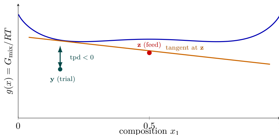
Figure 57: Michelsen's tangent-plane stability test, read off the molar-Gibbs-of-mixing surface g(x) . Draw the hyperplane tangent to g at the feed \mathbf{z} (orange). The tangent-plane distance \text{tpd}(\mathbf{y}) is the vertical gap between the surface and that tangent, measured at a trial composition \mathbf{y} . Here the surface dips below the tangent near \mathbf{y} : \text{tpd}(\mathbf{y}) < 0 , which proves the single feed is unstable and a liquid-liquid split exists — and that \mathbf{y} is a ready-made guess for the incipient phase. A feed is stable (one phase) iff \text{tpd} \geq 0 everywhere. At a converged stationary point this whole picture collapses to one number, \text{tm} = 1 - \sum_i Y_i , the quantity michelsenTPD actually tests.
