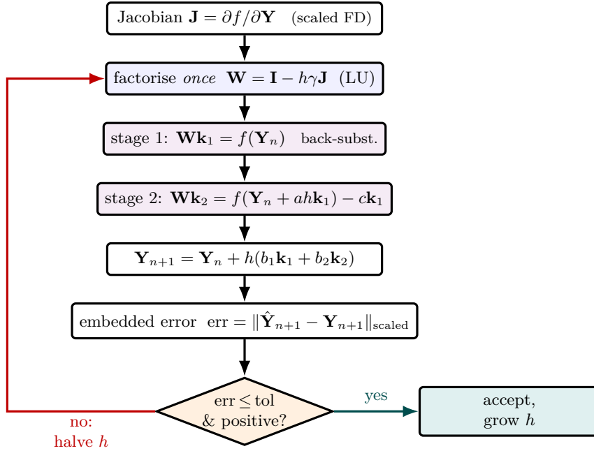
Figure 91: One adaptive step of Rosenbrock23, the stiff integrator ( src/solver/ODE/Rosenbrock23 ). The key economy is the blue box: the matrix \mathbf{W} = \mathbf{I} - h\gamma\mathbf{J} is LU-factorised once per step and then reused by both linear stages (violet) — each stage is just a back-substitution, and because the stages are linear in the unknowns there is no inner Newton loop (the trait that keeps the code glass-box, unlike backward-Euler/BDF). The order-2 update and an embedded order-3 estimate \hat{\mathbf{Y}} differ by the local error, which drives the controller: if the (component-scaled) error is within tolerance and no concentration went negative, the step is accepted and h grows; otherwise h is halved, \mathbf{W} refactored, and the step retried (red). L-stability means a stiff transient is absorbed , not rung — where fixed-step RK4 would overflow on the Robertson benchmark.
