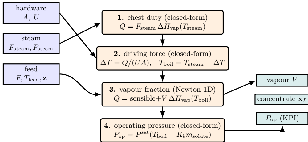
Figure 54: The credo evaporator solves four equations in order , and the operating pressure P_{\text{op}} — which the student never writes — falls out at the end. Only hardware ( A, U ) and the streams enter (blue). 1. The condensing steam fixes the duty Q . 2. The hardware turns Q into a driving force \Delta T and hence the boiling temperature T_{\text{boil}} , set by chest and geometry alone . 3. A single Newton-1D closes the process-side energy balance for the vapour flow V . 4. The Antoine curve, corrected for boiling-point elevation K_b m , inverts T_{\text{boil}} back to the pressure the vessel must sit at. No mode switch, no P_{\text{op}} in the dict — the crown jewel of the credo is a computed output, not an input.
