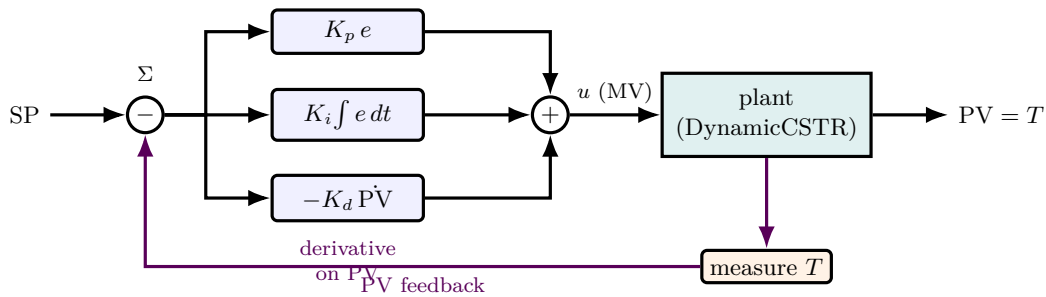
Figure 85: The ideal-form PID loop Choupo’s PIDController implements ( src/control/PIDController ). The summing junction forms the error e = SP - PV ; three parallel terms act on it — proportional ( K_p e , the present), integral ( K_i \int e dt , the accumulated past, killing offset) and derivative (the anticipated future) — and their sum is the manipulated variable u driving the plant (here T_{\text{jacket}} of the dynamic CSTR). The measured T is fed back (violet) to close the loop. Two Choupo choices are visible: the derivative tap reads PV directly, not e , so an operator’s set-point step produces no derivative “kick”; and the integral term is governed by the anti-windup gate of Figure 86.
