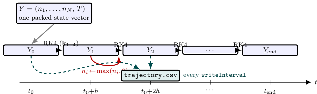
Figure 81: Time-marching with a packed state vector (Eq. 498). Every state variable of the vessel — the N component mole numbers and the temperature — is packed into one vector Y , and the generic RK4 stencil (Figure 46) advances it one fixed step h = \text{deltaT} at a time along the instant ladder Y_0 \rightarrow Y_1 \rightarrow \dots . After each step the mole numbers are projected onto the non-negative orthant ( n_i \leftarrow \max(n_i, 0) , red) to absorb the small negative drifts RK4 produces near depletion. The solver does not store every instant: it samples the trajectory to trajectory.csv every writeInterval seconds (green). The same machinery serves the isothermal batch ( Y = \mathbf{n} ), the adiabatic batch ( Y = (\mathbf{n}, T) , Section 2) and the dynamic CSTR (Section 4) — only f(Y) changes.
