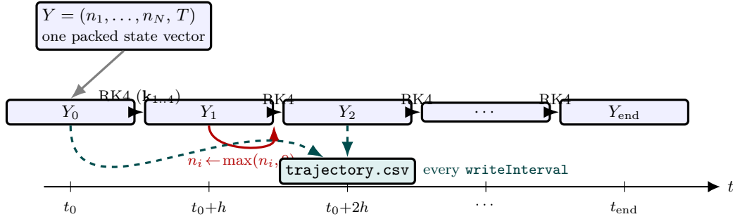
Figure 81: Time-marching with a packed state vector (Eq. 524). Every state variable of the vessel — the N component mole numbers and the temperature — is packed into one vector Y , and the generic RK4 stencil (Figure 46) advances it one fixed step h = \text{deltaT} at a time along the instant ladder Y_0 \rightarrow Y_1 \rightarrow \dots . After each step the mole numbers are projected onto the non-negative orthant ( n_i \leftarrow \max(n_i, 0) , red) to absorb the small negative drifts RK4 produces near depletion. The solver does not store every instant: it samples the trajectory to trajectory.csv every writeInterval seconds (green). The same machinery serves the isothermal batch ( Y = \mathbf{n} ), the adiabatic batch ( Y = (\mathbf{n}, T) , Section 2) and the dynamic CSTR (Section 4) — only f(Y) changes.
