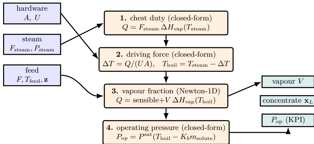
Figure 55: The credo evaporator solves four equations in order , and the operating pressure P_{\text{op}} — which the student never writes — falls out at the end. Only hardware ( A, U ) and the streams enter (blue). 1. The condensing steam fixes the duty Q . 2. The hardware turns Q into a driving force \Delta T and hence the boiling temperature T_{\text{boil}} , set by chest and geometry alone . 3. A single Newton-1D closes the process-side energy balance for the vapour flow V . 4. The Antoine curve, corrected for boiling-point elevation K_b m , inverts T_{\text{boil}} back to the pressure the vessel must sit at. No mode switch, no P_{\text{op}} in the dict — the crown jewel of the credo is a computed output, not an input.
