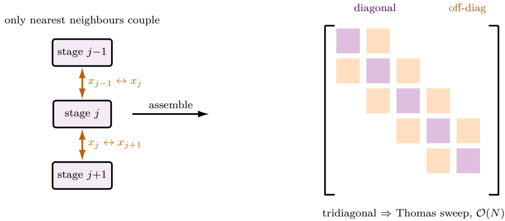
Figure 66: Why a column’s component balance is tridiagonal . Around stage j the steady balance ties only three liquid compositions — x_{j-1} descending in, x_j leaving, x_{j+1} rising in (one species shown). Because each stage couples to just its two neighbours , stacking the N balances gives a matrix with non-zeros only on the main diagonal and the two adjacent ones: a banded, tridiagonal system, one per component. Such a system is solved exactly by the Thomas algorithm in a single forward-then-backward sweep at \mathcal{O}(N) cost — no general matrix inversion — which is what Wang–Henke’s inner step and the absorber cascade both exploit. The simultaneous MESH Newton keeps the same band structure in its Jacobian, which is why even the rigorous column stays cheap per iteration.
