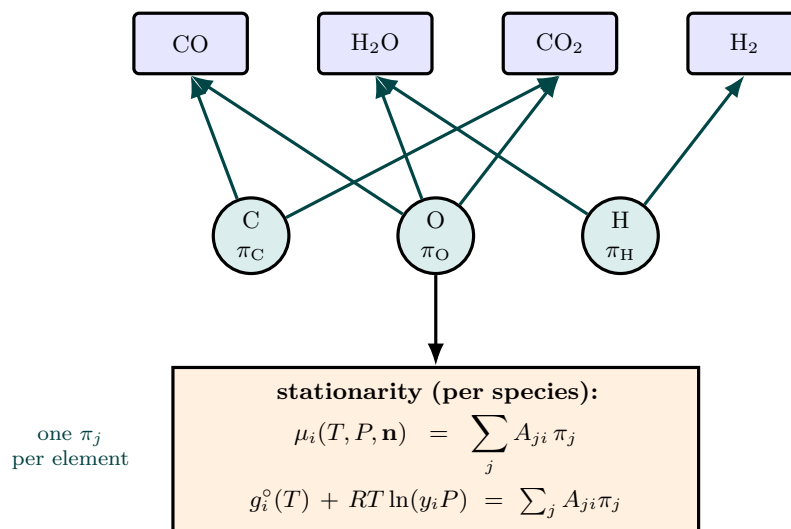
Figure 64: The Gibbs reactor never enumerates reactions. Instead it attaches one Lagrange multiplier \pi_j — an element chemical potential — to each conserved element (C, O, H ..., teal circles), and the atom-balance constraints \mathbf{A} \mathbf{n} = \mathbf{b} wire every species (blue) to the elements it contains. At the constrained minimum of G each species' chemical potential equals the sum of its element potentials, \mu_i = \sum_j A_{ji} \pi_j (orange box). That is N stationarity equations plus M element balances — a small Newton system in (\mathbf{n}, \boldsymbol{\pi}) — replacing the combinatorial mess of “which reactions occur”. The water-gas-shift species shown here resolve themselves automatically.
