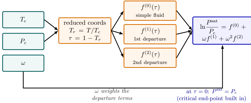
Figure 4: Ambrose–Walton turns the three corresponding-states constants an estimate already produces ( T_c , P_c , \omega , teal) into the whole saturation curve, with no measured vapour pressure. The reduced temperature feeds three universal shape functions f^{(0)} , f^{(1)} , f^{(2)} (orange, the same for every fluid); the acentric factor \omega weights the two departure terms and the sum returns \ln(P^{\text{sat}}/P_c) (blue). Because every f^{(i)} vanishes at \tau = 1 - T_r = 0 , the curve passes through P^{\text{sat}} = P_c at the critical point by construction —which is exactly what makes a freshly estimated component flashable.
