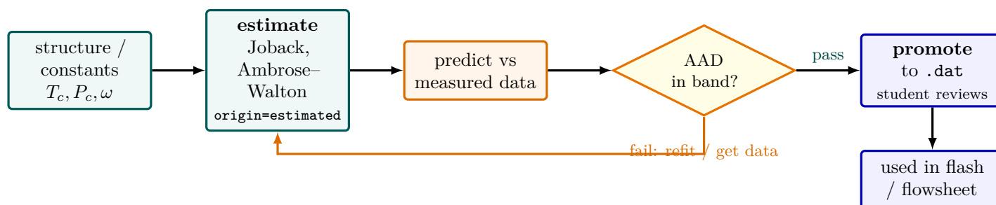
Figure 5: The glass-box property pipeline: estimate , then validate , then promote . From a molecular structure or three critical constants a group-contribution or corresponding-states method produces a value tagged origin=estimated (teal). Before it is trusted it is compared against measured data and scored by the average-absolute-deviation (AAD); the gate (yellow) is the project’s no-silent-crutch rule applied to data quality. Only a value that clears its accuracy band is promoted into the curated .dat the student reviews (blue) and the solver then reads. A failing estimate loops back to be refitted or replaced by laboratory data—it is never silently used.
