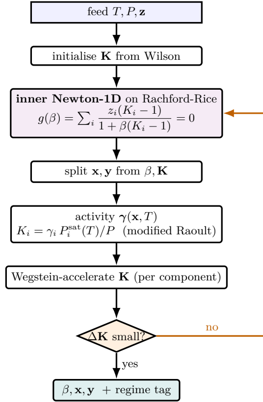
Figure 51: The isothermal V–L flash is two nested loops . The inner loop (violet) is a Newton-1D that solves the Rachford–Rice equation for the vapour fraction \beta at the current K -values — a clean monotone root. The outer loop (orange) updates the K -values: from the trial split it re-evaluates the activity coefficients \gamma_i(\mathbf{x}, T) , rebuilds K_i = \gamma_i P_i^{\text{sat}}(T)/P through modified Raoult, and Wegstein-accelerates them. When the K -values stop moving the two loops are mutually consistent and the flash is converged; the final \beta also classifies the regime (subcooled \beta < 0 , two-phase 0 \leq \beta \leq 1 , superheated \beta > 1 ). For an ideal system the activity step is a no-op and only the inner loop runs once — the same code, fewer passes.
