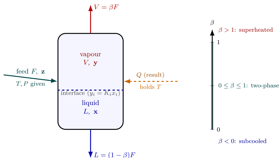
Figure 49: The flash drum as hardware. One feed ( F, \mathbf{z} ) at the specified ( T, P ) enters and disengages into a vapour V = \beta F off the top and a liquid L = (1 - \beta)F off the bottom, the two phases meeting at the interface where y_i = K_i x_i . The vapour fraction \beta = V/F is not an input — it is the Rachford–Rice root forced by the mass balance. The duty Q (dashed, orange) is whatever heat must cross the wall to hold T while part of the feed changes phase: a result of the converged energy balance, shown as a stream, never a hidden number. The ruler on the right reads \beta back as a regime tag: a \beta outside [0, 1] is the honest signal that the feed is single-phase (subcooled or superheated) at the chosen T, P .
