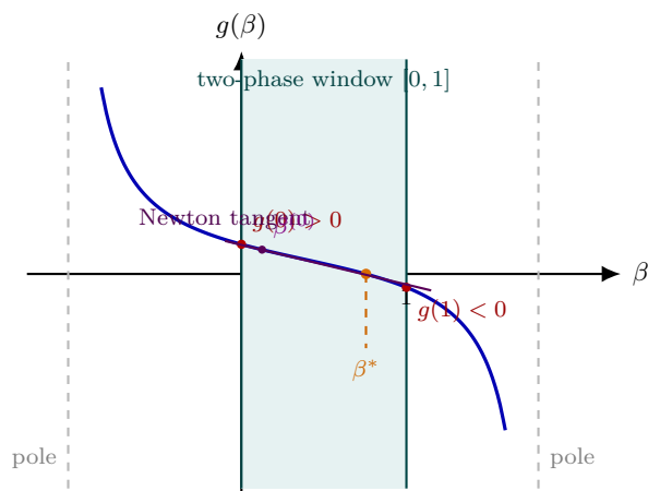
Figure 25: Why Rachford–Rice is tame. Each term has a pole where 1 + \beta(K_i - 1) = 0 ; for a genuine two-phase mixture all the poles lie outside the physical window [0, 1] (shaded), so on that window g is a single, smooth, strictly decreasing branch ( g'(\beta) < 0 always). When a split exists the endpoints straddle zero — g(0) > 0 , g(1) < 0 — guaranteeing exactly one root \beta^* in (0, 1) . Monotone plus a sign change is the textbook recipe for a trouble-free Newton: the tangent from any interior \beta^{(0)} slides to \beta^* and converges quadratically. If the endpoints share a sign, the root is pushed outside [0, 1] — the subcooled / superheated case the flash reports honestly.
