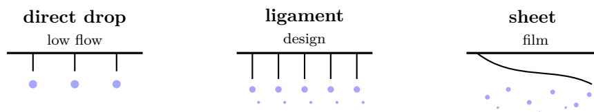
Figure 79: The three break-up regimes at a rotary wheel's rim as the feed rate rises (after Christensen & Steely; Lefebvre & McDonell, Atomization and Sprays ). Direct drop : discrete, near-monodisperse drops shed one at a time. Ligament : radial jets break by Rayleigh instability into main drops + satellites — the industrial regime. Sheet/film : a continuous sheet overhangs the rim and breaks irregularly — a broad, coarse spray. Turning the feed up to raise throughput can silently cross ligament→sheet and widen the powder.
