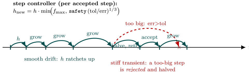
Figure 89: The adaptive step-size trajectory of Rosenbrock23 over several steps (the per-step internals are in Figure 92). On the smooth drift the embedded error stays well below tolerance, so after each accepted step the controller grows h (green arcs ratchet wider) — h_{\text{new}} = h \cdot \min(f_{\text{max}}, \text{safety}(\text{tol}/\text{err})^{1/3}) for the order-2/3 pair. When the solution hits a stiff transient a trial step overshoots tolerance: it is rejected ( \times ), h is halved, the matrix \mathbf{W} refactorised, and the step retried until it is accepted (red dashed \rightarrow short green arcs). The integrator thus spends large steps where nothing happens and small steps exactly where the action is — automatically, from the embedded error alone.
