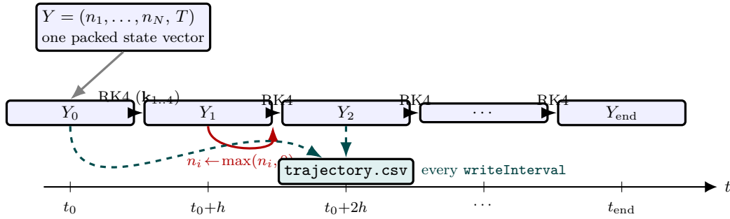
Figure 81: Time-marching with a packed state vector (Eq. 520). Every state variable of the vessel — the N component mole numbers and the temperature — is packed into one vector Y , and the generic RK4 stencil (Figure 46) advances it one fixed step h = \text{deltaT} at a time along the instant ladder Y_0 \rightarrow Y_1 \rightarrow \dots . After each step the mole numbers are projected onto the non-negative orthant ( n_i \leftarrow \max(n_i, 0) , red) to absorb the small negative drifts RK4 produces near depletion. The solver does not store every instant: it samples the trajectory to trajectory.csv every writeInterval seconds (green). The same machinery serves the isothermal batch ( Y = \mathbf{n} ), the adiabatic batch ( Y = (\mathbf{n}, T) , Section 2) and the dynamic CSTR (Section 4) — only f(Y) changes.
