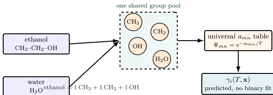
Figure 13: UNIFAC’s central idea, drawn: a molecule is dissolved into a multiset of functional groups (ethanol = CH 3 +CH 2 +OH), and the mixture is treated as a solution of those groups rather than of molecules. A CH 2 is assumed to interact with H 2 O the same way in every molecule it appears in — the group-additivity hypothesis — so a single universal a_{mn} table ( \Psi_{mn} = e^{-a_{mn}/T} ) serves all of chemistry. That is what turns UNIQUAC’s fitted residual term into a prediction : feed in the group counts and out comes \gamma_i(T, \mathbf{x}) for a binary nobody ever measured. The price is proximity effects and isomers the group count cannot see (see the limits).
