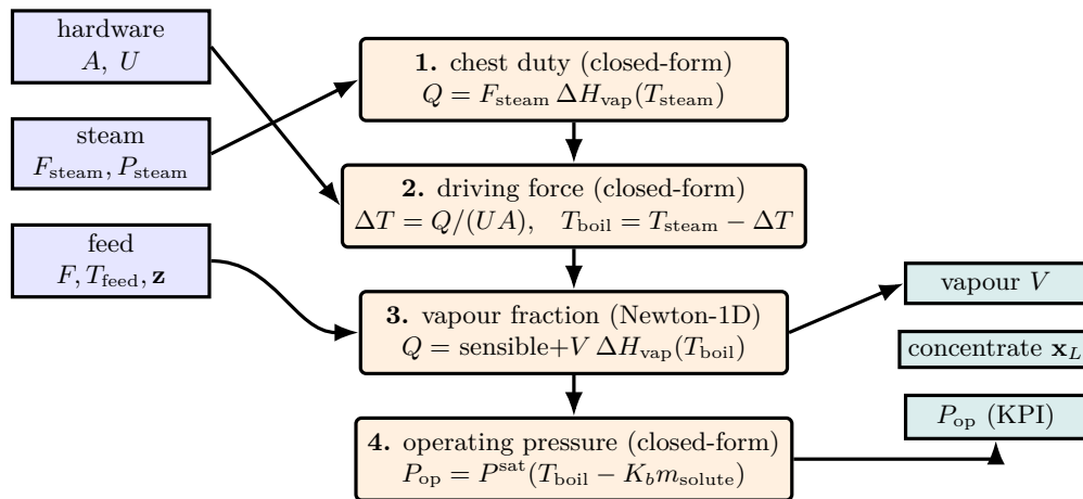
Figure 55: The credo evaporator solves four equations in order , and the operating pressure P_{\text{op}} — which the student never writes — falls out at the end. Only hardware ( A, U ) and the streams enter (blue). 1. The condensing steam fixes the duty Q . 2. The hardware turns Q into a driving force \Delta T and hence the boiling temperature T_{\text{boil}} , set by chest and geometry alone . 3. A single Newton-1D closes the process-side energy balance for the vapour flow V . 4. The Antoine curve, corrected for boiling-point elevation K_b m , inverts T_{\text{boil}} back to the pressure the vessel must sit at. No mode switch, no P_{\text{op}} in the dict — the crown jewel of the credo is a computed output, not an input.
