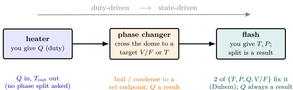
Figure 52: Three single-vessel thermal units, ordered by what the student specifies. The heater is duty-driven: you furnish Q and the outlet temperature follows — no phase split is even asked. The flash is state-driven: you fix two of \{T, P, Q, V/F\} (Duhem’s rule), and the vapour–liquid split is the result, with Q always an output, never an input key. The phase changer sits between them — a boiler/condenser that crosses the saturation dome to a set endpoint (a target V/F or T ), reporting the duty it took. Reading the units this way — duty-driven on the left, state-driven on the right — keeps the degrees of freedom straight and avoids the classic “is Q an input or an output?” confusion.
