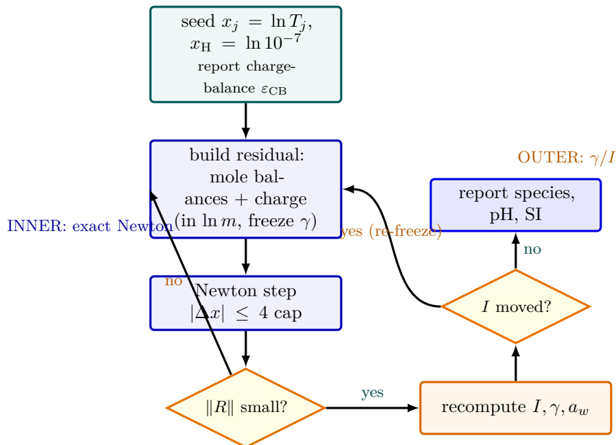
Figure 17: The speciation solver as a two-loop machine—the same freeze-the-slow-coupling pattern as a recycle tear. The inner loop (blue) is an exact Newton on the mole balances (plus electroneutrality when the pH is solved), written in \ln m so molalities stay positive and the mass-action laws turn linear; each step is capped at |\Delta x| \leq 4 so the iteration cannot leap out of its basin. The outer loop (orange) freezes the activity coefficients, solves the inner system exactly, then re-evaluates \gamma and a_w at the new ionic strength, repeating until I stops moving. Before any of it runs, the charge-balance error \varepsilon_{CB} is reported (teal)—a solved pH is no better than the analysis it balances.
