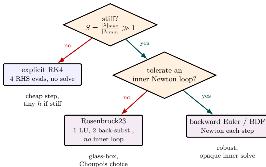
Figure 85: The integrator decision tree. If the eigenvalue spread S is \mathcal{O}(1) the system is non-stiff and explicit RK4 wins — four right-hand-side evaluations, nothing solved. Once S \gg 1 an explicit method is hostage to the dead fast mode (Figure 87), so an implicit method is required, and the only remaining question is whether to pay for an inner Newton iteration. Choupo takes the left branch: the linearly-implicit Rosenbrock23 keeps full implicit stability but replaces the inner loop with one LU factorisation reused by two back-substitutions — the trait that keeps the stiff solver as readable as the non-stiff one.
