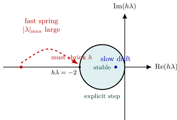
Figure 87: The stability region of an explicit step (forward Euler shown: the disc |1 + h\lambda| \leq 1 , centre -1 , radius 1 ). Every eigenmode \lambda of the Jacobian, multiplied by the step h , must land inside the disc or that mode is amplified and the integration blows up. A slow drift mode (blue) sits comfortably inside for almost any h ; but the fast spring (red, large |\lambda|_{\max} ) forces h \lesssim 2/|\lambda|_{\max} to drag it back across the boundary at h\lambda = -2 — even after that mode has died and stopped contributing to the answer. That is stiffness: the dead fast mode, not accuracy, sets the step. The implicit cure (Rosenbrock23, Figure 89) has no such boundary in the left half-plane.
