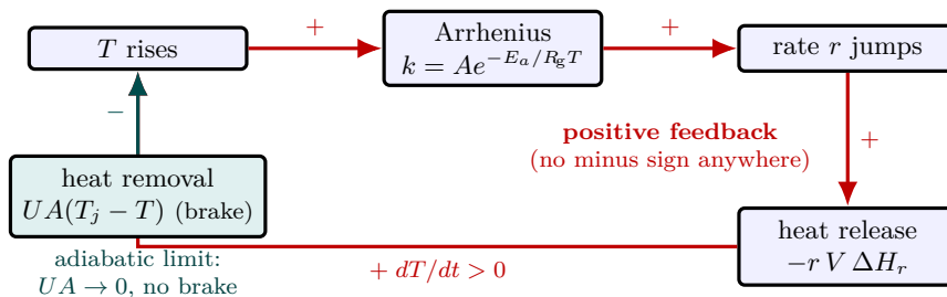
Figure 79: The thermal-runaway feedback loop of an adiabatic batch reactor. A rise in T lifts the Arrhenius rate constant k exponentially, which raises the reaction rate r , which releases more heat, which raises T further — every arrow carries a “+”, so the loop is positive feedback with no restoring term. The only brake is heat removal UA(T_j - T) (green); in the adiabatic limit UA \rightarrow 0 it vanishes and, once the “thermal Jacobian” J_{T,T} \propto E_a/(R_g T^2 \sum_i n_i C_{p,i}) exceeds the (here zero) loss term, the system has no stable steady state and must run away. The case batch02_adiabatic sits on this side: \sim 200 s of quiescence while r is tiny, then the Arrhenius factor catches and T climbs 345 \rightarrow 482 K in \sim 100 s.
