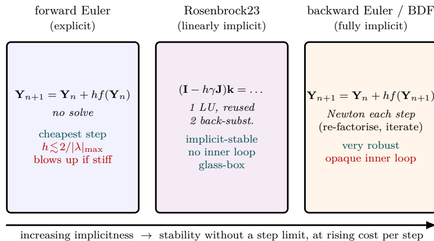
Figure 88: Three rungs of implicitness for the stiff IVP d\mathbf{Y}/dt = f(\mathbf{Y}) . Forward Euler (left) solves nothing per step but is hostage to the stability limit h \lesssim 2/|\lambda|_{\max} and overflows on a stiff system. Backward Euler/BDF (right) is unconditionally stable but pays an inner Newton iteration every step — robust, but the iteration is the opaque box Choupo wants to avoid. Rosenbrock23 (centre) is the linearly-implicit compromise: it linearises f once, assembles \mathbf{W} = \mathbf{I} - h\gamma\mathbf{J} , factorises it once , and reuses the factorisation across both stages — keeping full implicit stability without an inner loop. That is why Choupo’s stiff solver (Figure 89) reads almost as plainly as its RK4.
