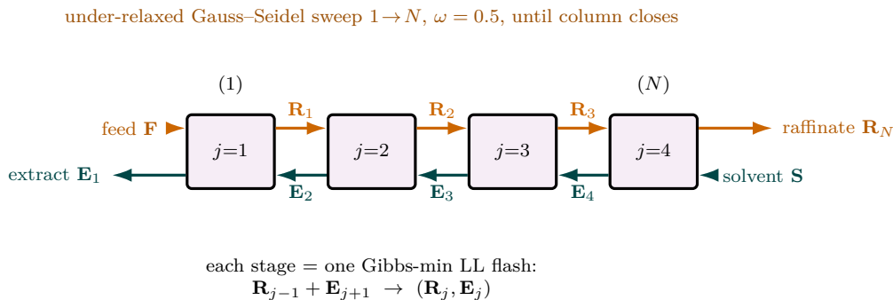
Figure 61: The counter-current extraction cascade. Feed \mathbf{F} enters stage 1 and fresh solvent \mathbf{S} enters stage N ; the feed-derived raffinate (orange) flows 1 \rightarrow N while the solvent-rich extract (teal) flows N \rightarrow 1 , so the leaving extract has met the richest feed and the leaving raffinate the cleanest solvent. Each stage is exactly one liquid–liquid Gibbs-min flash (Fig. 60’s two-liquid cousin): it takes the combined inlet \mathbf{R}_{j-1} + \mathbf{E}_{j+1} and splits it into the two equilibrium liquids. Because the two directions are coupled, the cascade is a fixed-point problem; Choupo tears it by under-relaxed Gauss–Seidel sweeps ( \omega = 0.5 , the raw update oscillates) and stops not on a noisy per-stage delta but on the honest test that what leaves the column equals what entered it.
