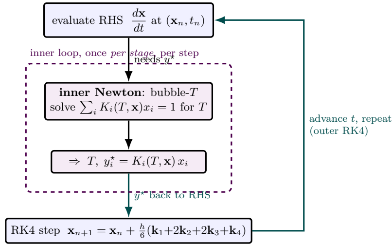
Figure 80: The nested-Newton pattern that recurs in every dynamic VLE problem, shown for Rayleigh batch distillation. The outer loop is RK4 marching the residue composition \mathbf{x} in time (blue). But each RK4 stage needs the equilibrium vapour y_i^* = K_i(T, \mathbf{x}) x_i , and that requires the boiling temperature — so a full inner Newton iteration (violet) solves the bubble-point condition \sum_i K_i(T, \mathbf{x}) x_i = 1 for T before the right-hand side can even be evaluated ( BubblePoint::compute used as a black box). The inner solve runs once per stage , four times per RK4 step; its result feeds the outer step, time advances, and the whole thing repeats. The same Newton-inside-RK4 structure drives the dynamic flash and every moving-VLE unit op.
