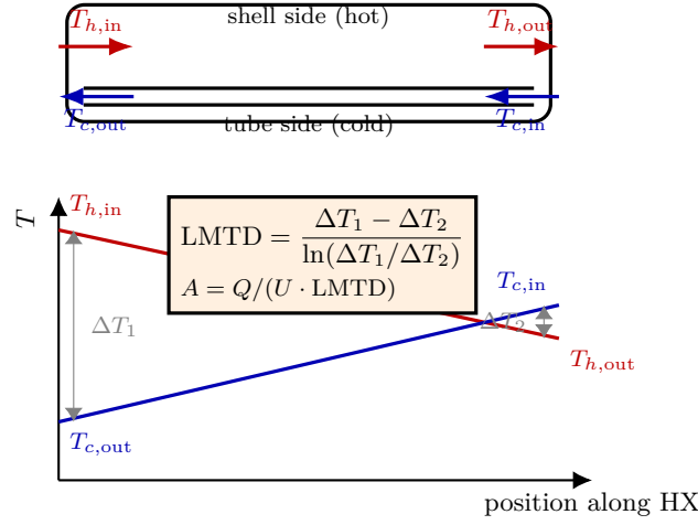
Figure 77: The shell-and-tube sizing picture. Top: a single-pass counter-current exchanger — hot stream in the shell, cold stream in the tubes, flowing in opposite directions. Bottom: the temperature profiles down the unit. The approach \Delta T is not constant — it is \Delta T_1 at one end and \Delta T_2 at the other — so the correct mean driving force is the log-mean LMTD, not the arithmetic average. Once the duty Q is known (a unit-op KPI) and U is supplied, the area is simply A = Q / (U \cdot \text{LMTD}) . Counter-current flow (cold rising against hot falling) keeps the approach open along the whole length — why it out-performs co-current for the same area.
