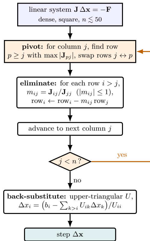
Figure 30: Gauss elimination with partial pivoting — the \sim 60 -line direct solver that every Newton step in the simulator calls to turn \mathbf{J} \Delta \mathbf{x} = -\mathbf{F} into a step. Column by column it first pivots (swaps in the row with the largest entry in the active column, the orange box) so the multipliers m_{ij} never exceed one in magnitude — the guard against round-off blow-up — then eliminates everything below the diagonal, leaving an upper-triangular system. When the last column is reached, one back-substitution sweep reads off \Delta \mathbf{x} from the bottom up. No matrix inverse is ever formed: the factorisation is both cheaper ( O(n^3/3) ) and steadier than \mathbf{J}^{-1} .
