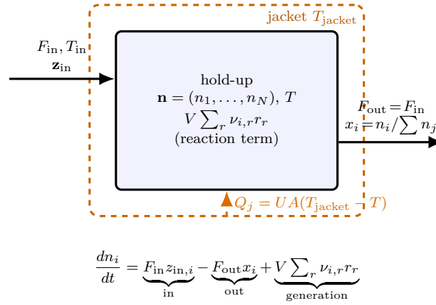
Figure 82: The continuous dynamic CSTR as a single 0-D well-mixed hold-up cell ( DynamicCSTR ). Unlike the steady CSTR of Section 5, the contents accumulate : the state \mathbf{Y} = (\mathbf{n}, T) evolves in time. Three currents cross the boundary of each component balance — convective inflow F_{\text{in}} z_{\text{in},i} , convective outflow F_{\text{out}} x_i at the tank composition (perfect mixing), and chemical generation V \sum_r \nu_{i,r} r_r — and the jacket adds a heat current Q_j = UA(T_{\text{jacket}} - T) to the energy balance. Constant liquid volume forces F_{\text{out}} = F_{\text{in}} , so total mass does not accumulate, yet composition does because x_i tracks n_i . The manipulated variables a controller may write (T_{\text{jacket}}, T_{\text{in}}, F_{\text{in}}) are exactly the labelled inlet and jacket quantities.
