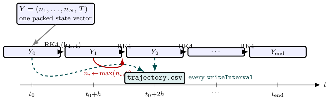
Figure 78: Time-marching with a packed state vector (Eq. 386). Every state variable of the vessel — the N component mole numbers and the temperature — is packed into one vector Y , and the generic RK4 stencil (Figure 45) advances it one fixed step h = \text{deltaT} at a time along the instant ladder Y_0 \rightarrow Y_1 \rightarrow \dots . After each step the mole numbers are projected onto the non-negative orthant ( n_i \leftarrow \max(n_i, 0) , red) to absorb the small negative drifts RK4 produces near depletion. The solver does not store every instant: it samples the trajectory to trajectory.csv every writeInterval seconds (green). The same machinery serves the isothermal batch ( Y = \mathbf{n} ), the adiabatic batch ( Y = (\mathbf{n}, T) , Section 2) and the dynamic CSTR (Section 4) — only f(Y) changes.
