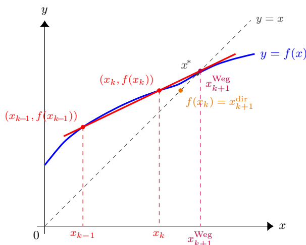
Figure 34: Geometric construction of one Wegstein step. Two prior iterates lie on the curve y=f(x) as (x_{k-1}, f(x_{k-1})) and (x_k, f(x_k)) . Their secant line (red) approximates f locally as an implicit linear model; the next iterate x_{k+1}^{\text{Weg}} is where this secant crosses the fixed-point diagonal y=x . Direct substitution would jump only as far as f(x_k) along the diagonal (orange) — visibly short of x^* — while the secant extrapolation lands almost exactly on the fixed point. For a linear f the secant coincides with the curve and Wegstein hits x^* in one step; for the non-linear f shown, the secant is a chord and one step gets within \sim 2\% of the root.
