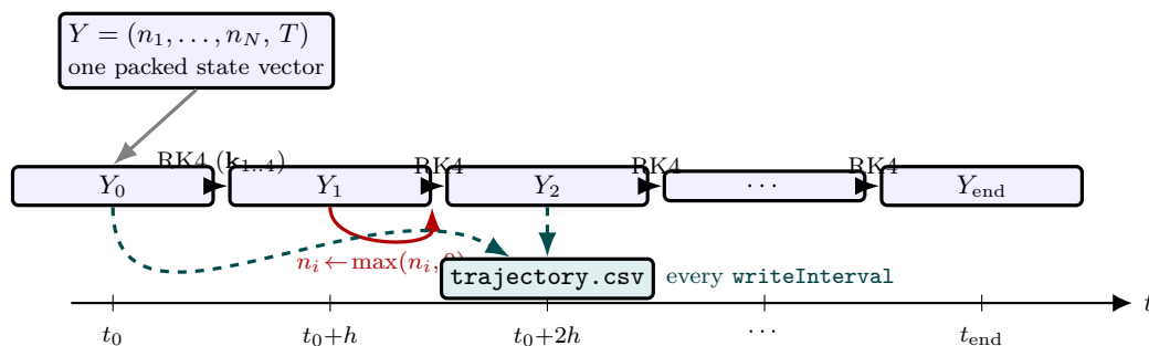
Figure 80: Time-marching with a packed state vector (Eq. 449). Every state variable of the vessel — the N component mole numbers and the temperature — is packed into one vector Y , and the generic RK4 stencil (Figure 45) advances it one fixed step h = \text{deltaT} at a time along the instant ladder Y_0 \rightarrow Y_1 \rightarrow \dots . After each step the mole numbers are projected onto the non-negative orthant ( n_i \leftarrow \max(n_i, 0) , red) to absorb the small negative drifts RK4 produces near depletion. The solver does not store every instant: it samples the trajectory to trajectory.csv every writeInterval seconds (green). The same machinery serves the isothermal batch ( Y = \mathbf{n} ), the adiabatic batch ( Y = (\mathbf{n}, T) , Section 2) and the dynamic CSTR (Section 4) — only f(Y) changes.
