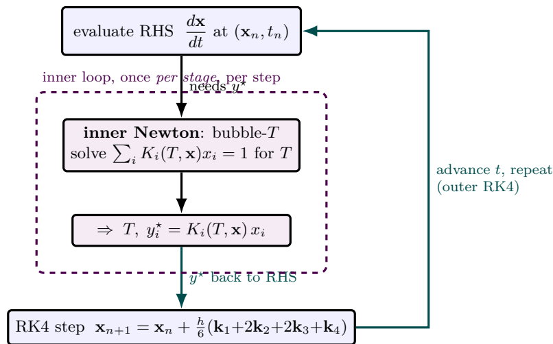
Figure 82: The nested-Newton pattern that recurs in every dynamic VLE problem, shown for Rayleigh batch distillation. The outer loop is RK4 marching the residue composition \mathbf{x} in time (blue). But each RK4 stage needs the equilibrium vapour y_i^* = K_i(T, \mathbf{x}) x_i , and that requires the boiling temperature — so a full inner Newton iteration (violet) solves the bubble-point condition \sum_i K_i(T, \mathbf{x}) x_i = 1 for T before the right-hand side can even be evaluated ( BubblePoint::compute used as a black box). The inner solve runs once per stage , four times per RK4 step; its result feeds the outer step, time advances, and the whole thing repeats. The same Newton-inside-RK4 structure drives the dynamic flash and every moving-VLE unit op.
