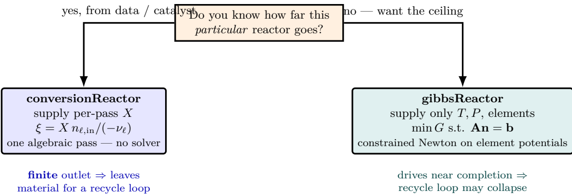
Figure 62: The two extreme reactor idealisations, and the conscious modelling choice between them. The conversion reactor answers “what does this reactor actually do?” — you supply the per-pass conversion X (known from a catalyst or plant data) and the outlet falls out of stoichiometry in a single algebraic pass, no solver. The Gibbs reactor answers “what is the best this chemistry could do?” — you supply nothing about extent, only T , P and the element inventory, and the outlet is the composition that minimises G subject to atom conservation. The recycle consequence is the deciding factor: a finite conversion leaves material for the loop, while equilibrium often drives to near-completion and the loop collapses.
