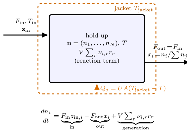
Figure 84: The continuous dynamic CSTR as a single 0-D well-mixed hold-up cell ( DynamicCSTR ). Unlike the steady CSTR of Section ??, the contents accumulate : the state \mathbf{Y} = (\mathbf{n}, T) evolves in time. Three currents cross the boundary of each component balance — convective inflow F_{\text{in}} z_{\text{in},i} , convective outflow F_{\text{out}} x_i at the tank composition (perfect mixing), and chemical generation V \sum_r \nu_{i,r} r_r — and the jacket adds a heat current Q_j = UA(T_{\text{jacket}} - T) to the energy balance. Constant liquid volume forces F_{\text{out}} = F_{\text{in}} , so total mass does not accumulate, yet composition does because x_i tracks n_i . The manipulated variables a controller may write (T_{\text{jacket}}, T_{\text{in}}, F_{\text{in}}) are exactly the labelled inlet and jacket quantities.
