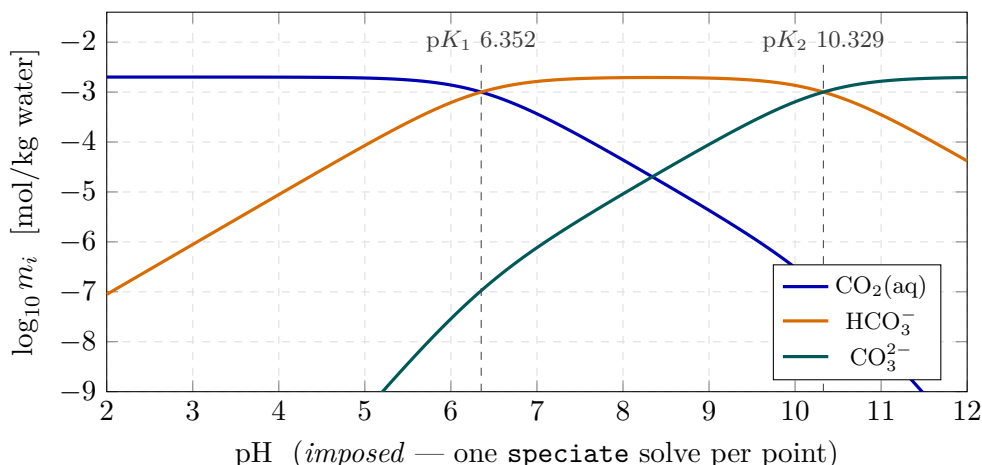
Figure 17: A distribution diagram of the carbonate system, 2 mmol/kg total carbonate: the three bands hand the material over at the two \text{p}K_a 's and separate by one decade per pH unit, (135), while a band two protons from the dominant one falls at two decades per unit. These curves are the closed form at \gamma_i = 1 , drawn from the two constants the curated records carry ( chemistry/C02aq-formation.dat , chemistry/C03-formation.dat ; USGS PHREEQC, public domain). A Choupo run does not draw this formula: its answer moves off these curves by the single-ion activity coefficients, by K_s(T) away from 25 °C, and by any ion pair the feed makes reachable (a sodium bicarbonate water forms \text{NaHCO}_3(\text{aq}) , which this expression has no term for). That gap is the reason the Explore lens plots the engine's own molalities instead — but the shape , and where the crossings sit, is this.
