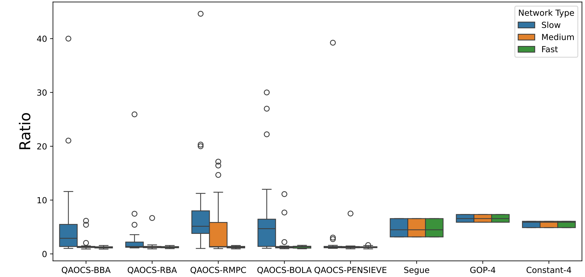
Switch Ratio(%) by Method and Network Type
