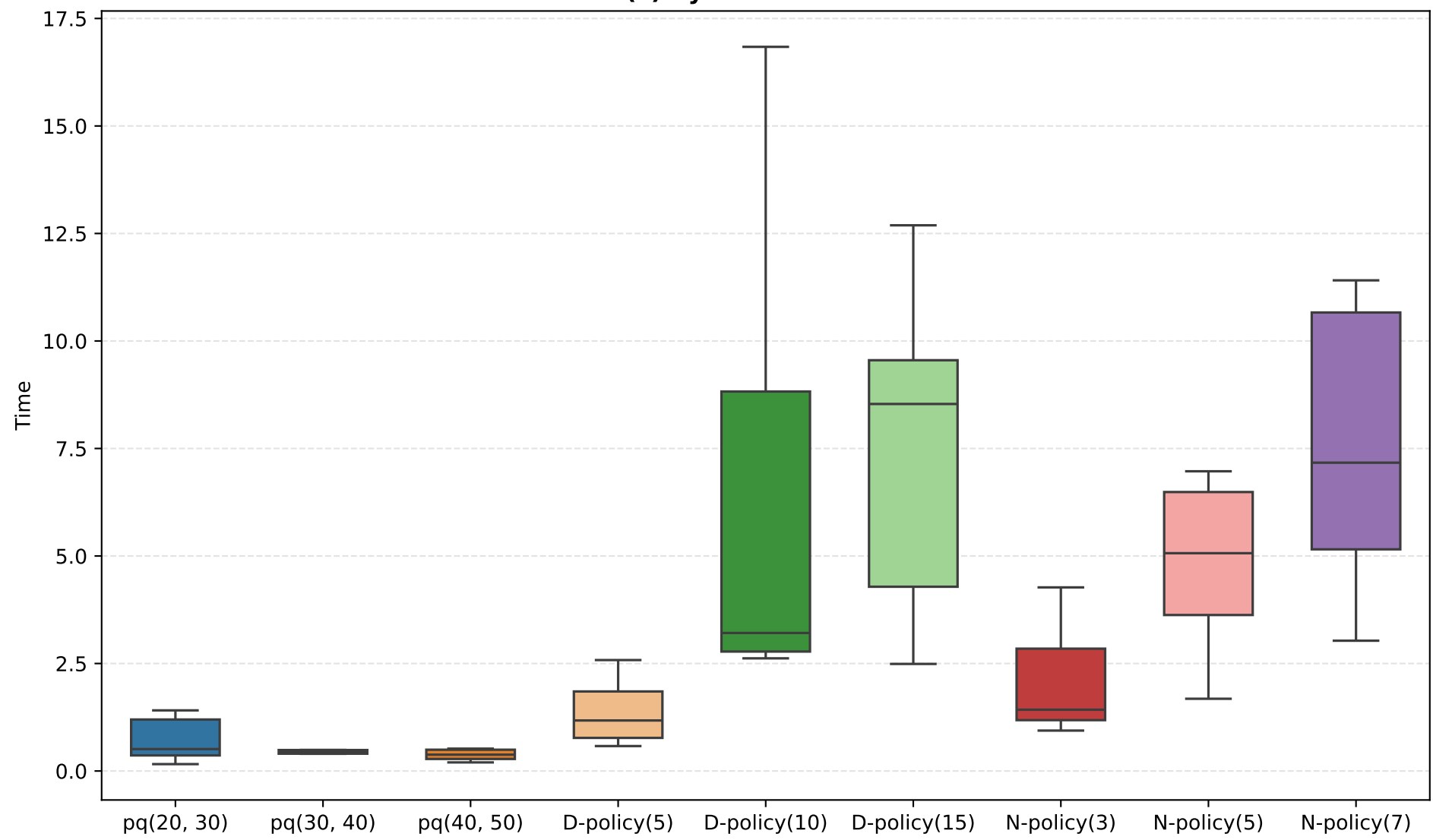
Stall Time(s) by Method — Slow network
