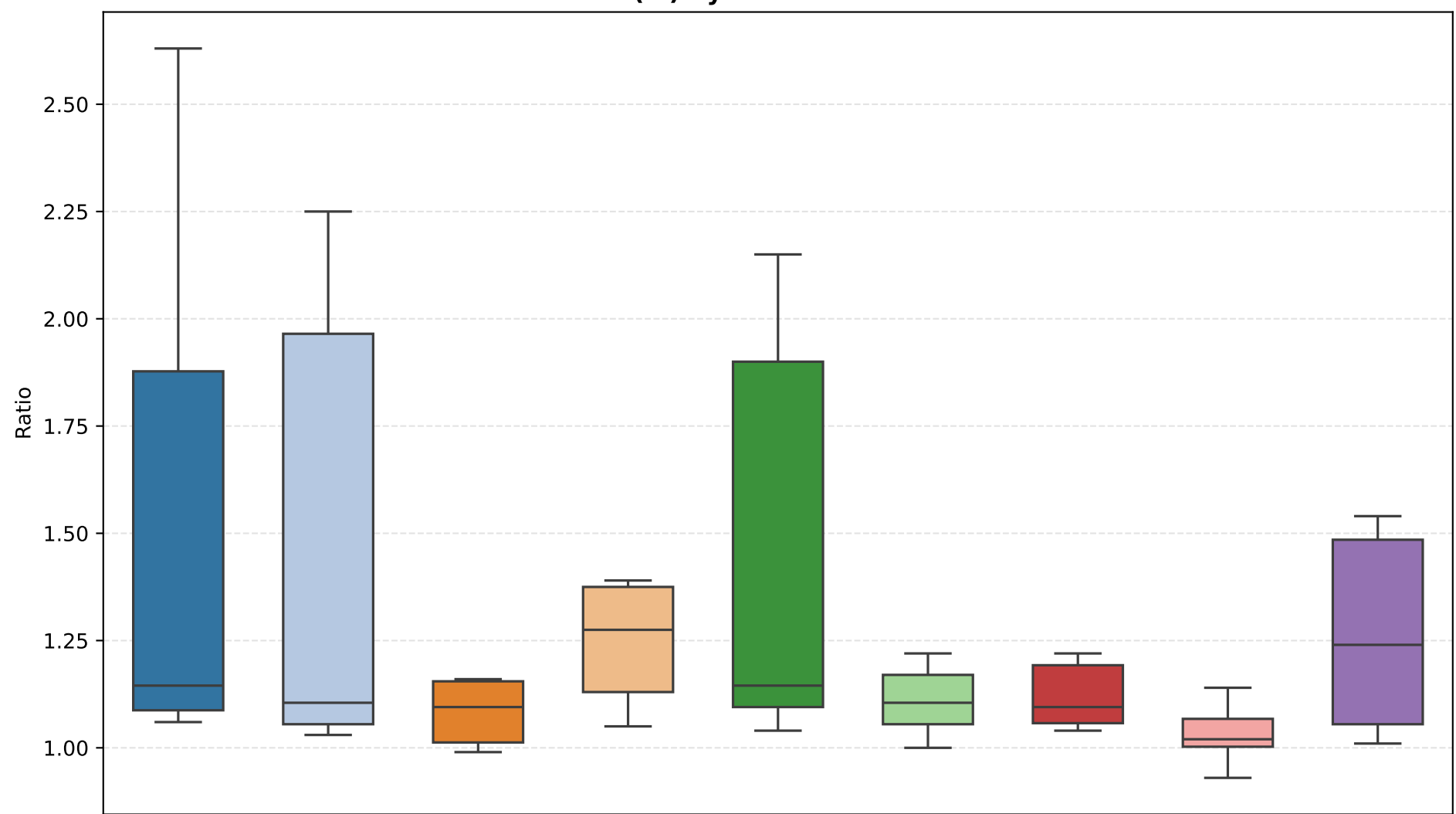
Stall Time(s) by Method — Slow network
