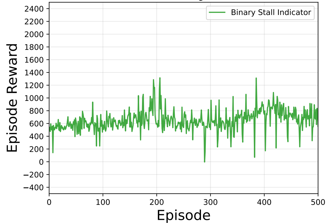
Raw Reward - Binary Stall Indicator
